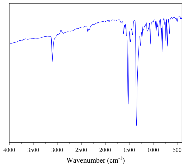
Figure S3. FTIR spectrum of 1b .
