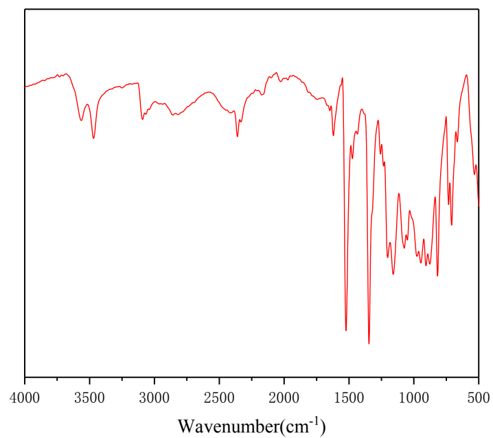
Figure S1. FTIR spectrum of 1a .
