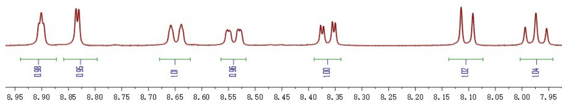
Figure S4. ^1\text{H} NMR spectrum of 1b
