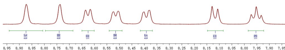
Figure S2. 1 H NMR spectrum of 1a .
