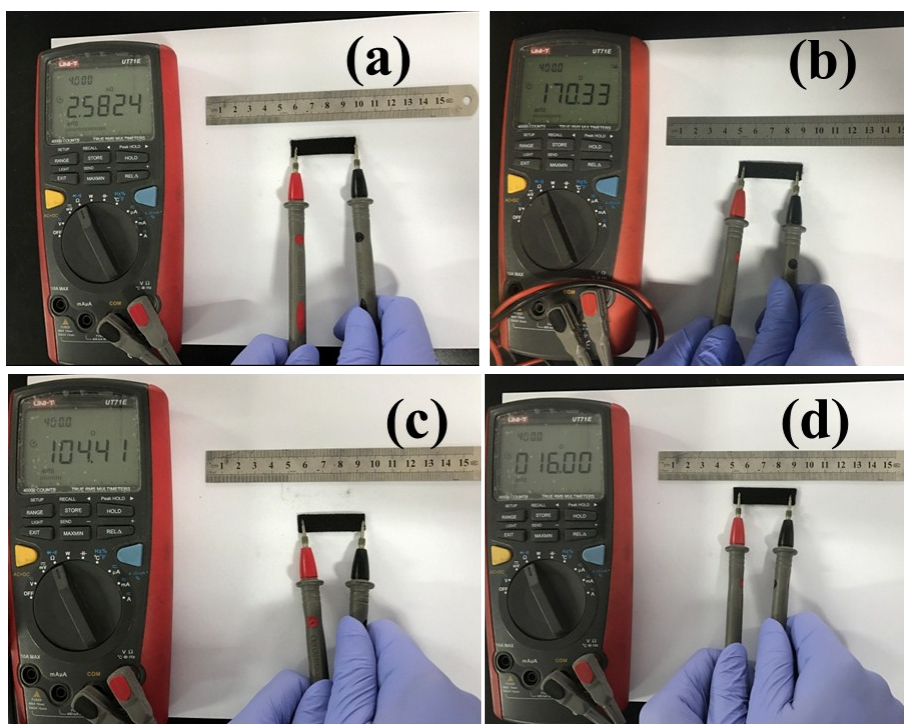
Figure S1 Photograph illustrating the ohm resistance of: (A) CF; (B) CF-800; (C) CF-900; (D) TCF.
