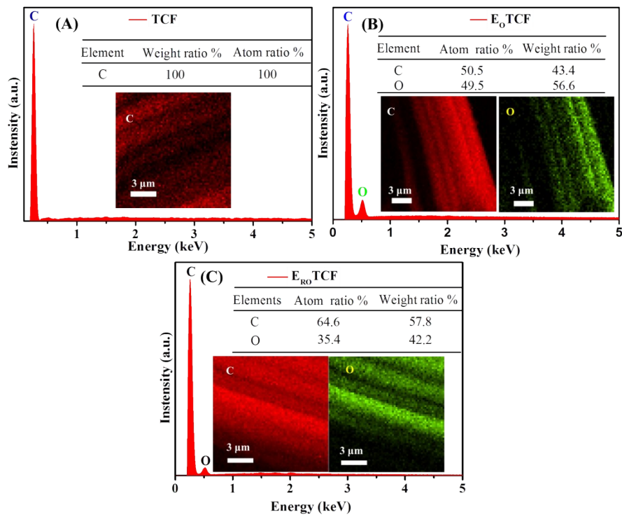
Figure S2 EDS patterns of (A) TCF, (B) E 0 TCF and (C) E RO TCF; the insets showing the corresponding EDS mapping images.
