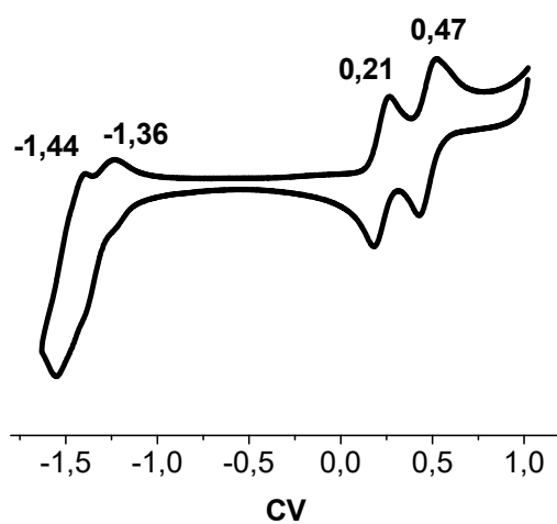
Figure S1 CV of compound 18a ( \text{CH}_2\text{Cl}_2 solution containing 0.1 M \text{TBAPF}_6 as the supporting electrolyte and \text{Fc}/\text{Fc}^+ as the internal standard).
