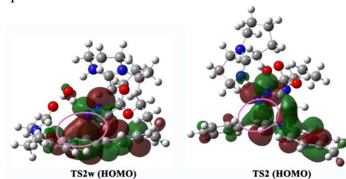
Figure S2. Orbital interactions in HOMOs of TS2w and TS2.
