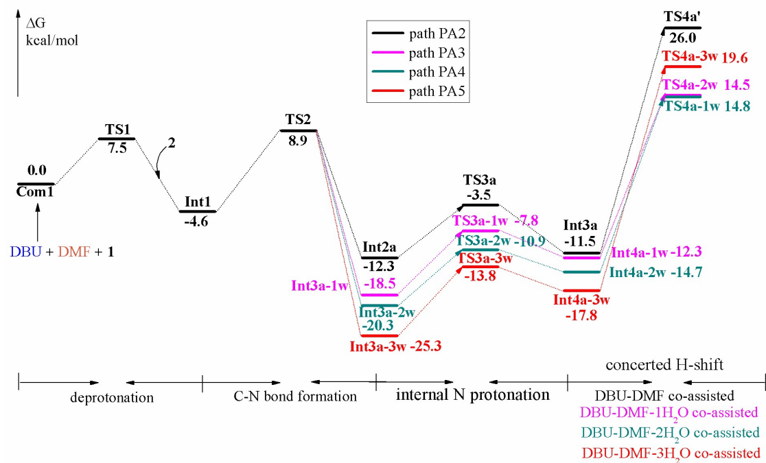
Figure S1. DFT computed energy surfaces for DBU-DMF co-assisted concerted H-shift pathway PA2, DBU-DMF-1H 2 O co-assisted concerted H-shift pathway PA3, DBU-DMF-2H 2 O co-assisted concerted H-shift pathway PA4, DBU-DMF-3H 2 O co-assisted concerted H-shift pathway PA5 in the solvent phase, and free energies are given in kcal/mol.
