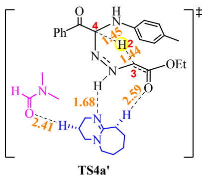
Scheme S1. Optimized structure of TS4a'.
