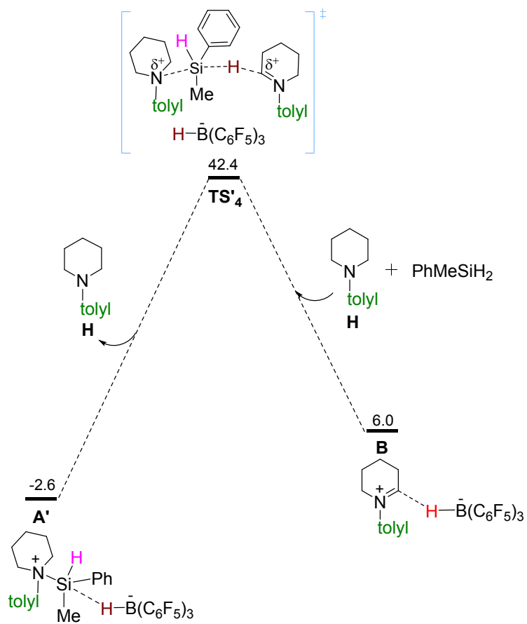
Figure S3. The formation of A' from B + \text{PhMeSiH}_2 + H via TS' 4 .
