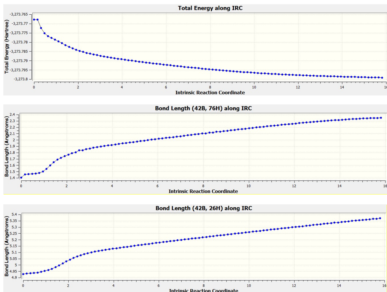
Figure S4. The energy, and (C 6 F 5 ) 3 B–H (hydride) and (C 6 F 5 ) 3 B–HSi(R)MePh distances along the IRC of TS 7 .
