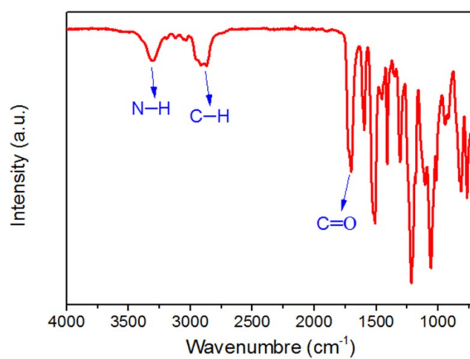
Fig. S2. FTIR spectrum of shape memory polyurethane (SMPU)
