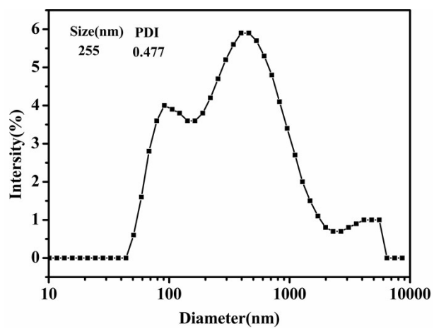
Fig. S1. Size distribution of samples with 0.5mol/L \text{Na}_2\text{HPO}_4
