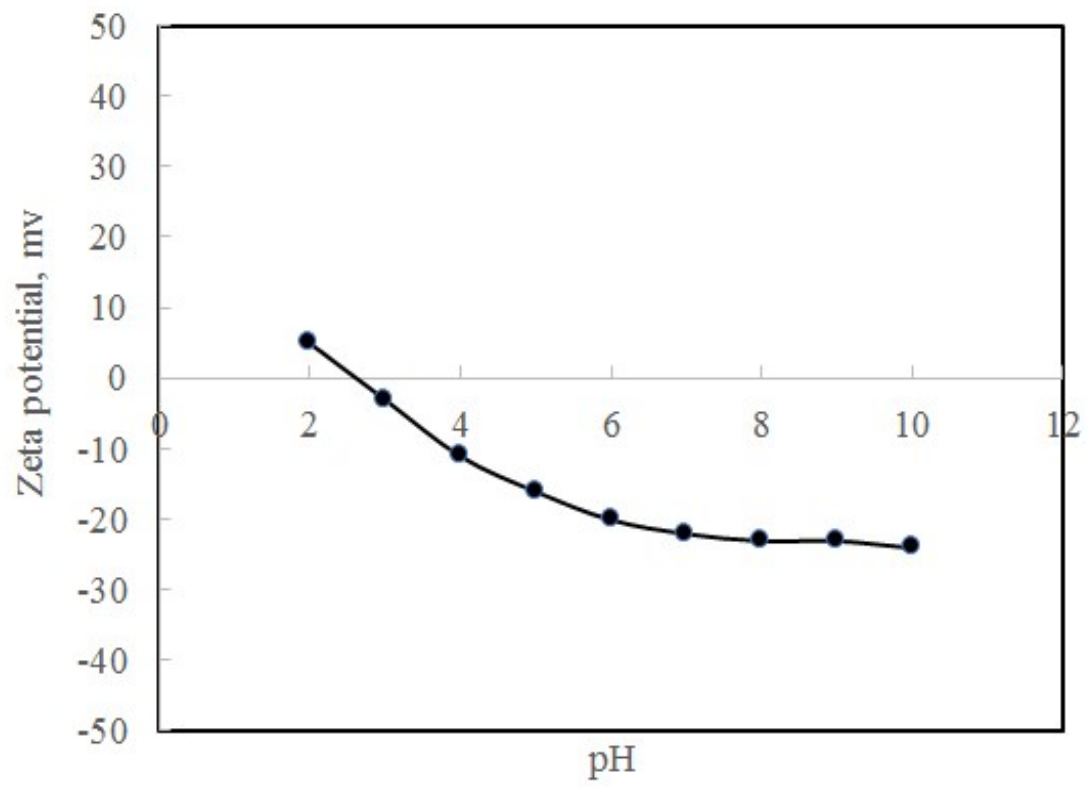
Fig.2 Zeta potential of the Zr-GP gel at different pH values
