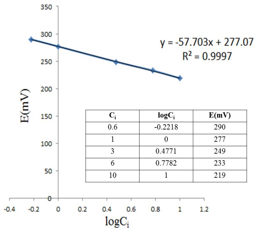
Fig.1 The calibration curve for the linear relationship between the standard concentration of fluoride ion and the electrode potential:
