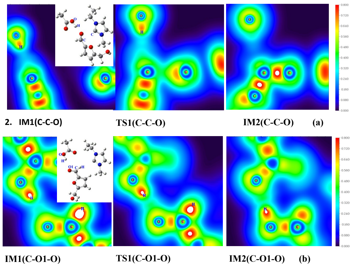
Fig. S1 Localized orbital locator (LOL) profiles of IM1 , TS1 and IM2 along (a) the C-C-O plane and (b) C-O1-O plane.
