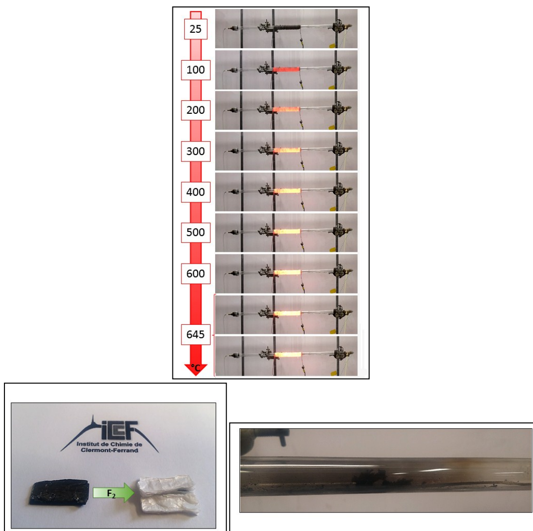
Figure SI 1: Picture of the experimental setup used for the fast thermal exfoliation of fluorinated carbons and pictures of the morphology of the FG before (white and thin) and after the exfoliation (black and exfoliated)
