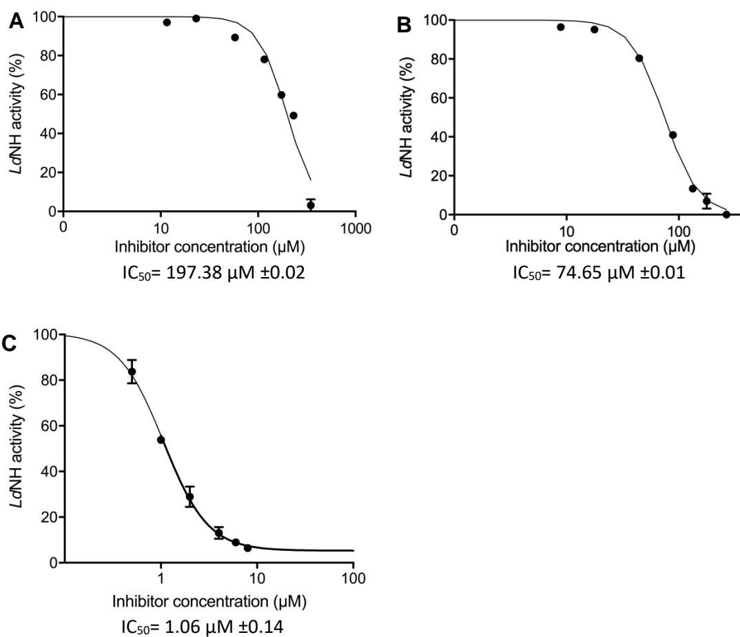
Figure S4. IC_{50} curves and values for compounds 1 (A), 2 (B) and 3 (C).
