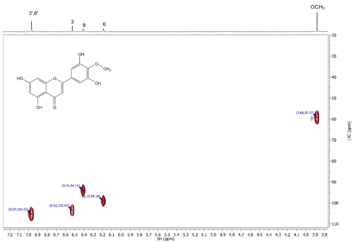
Figure S3. HSQC NMR spectrum of tricetin-4'-O-methyl flavone (3).
