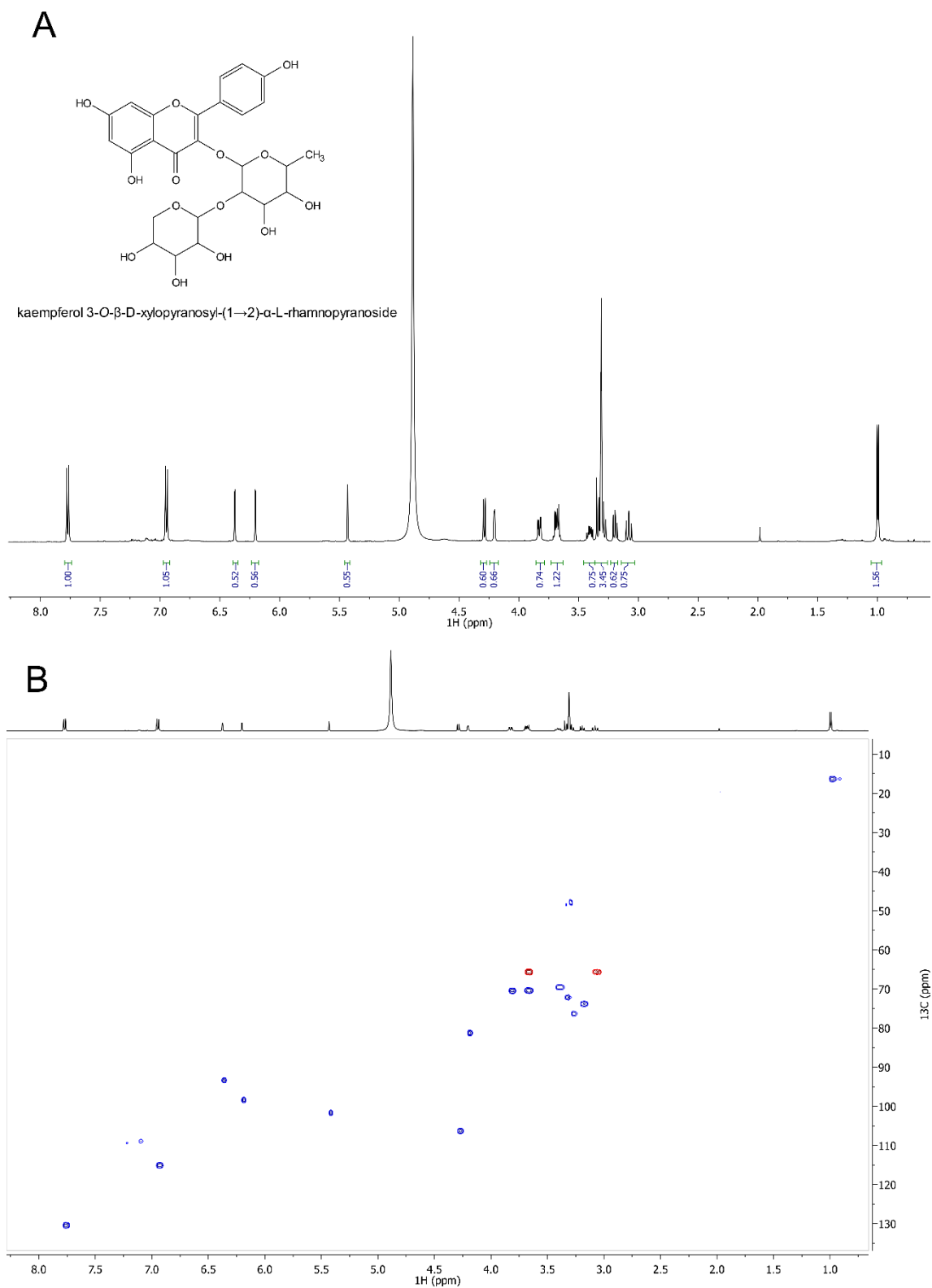
Figure S2. NMR spectra of kaempferol 3-O- \beta -D-xylopyranosyl-(1 \rightarrow 2)- \alpha -L-rhamnopyranoside ( 2 ). A) ^1\text{H} ; B) HSQC.
