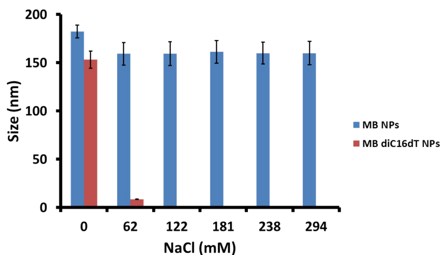
Figure S1: Size evolution of MB/diC16dT NPs (red) and MB-NPs (blue) at different concentrations of NaCl. Error bars represent standard deviation of three independent experiments.
