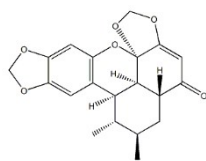
Supplementary Fig. 1. Chemical structure of sauchinone.
