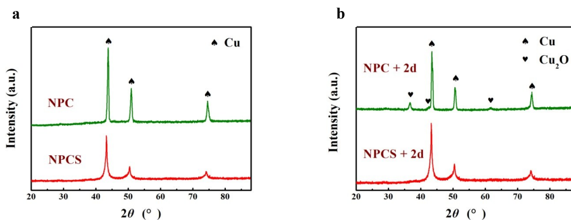
Fig. S2. XRD patterns of the dealloying samples which aged in air for (a) 0 days, (b) 2 days.
