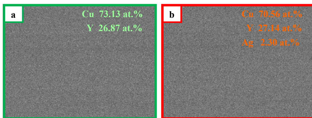
Fig. S1. SEM images and the corresponding EDS results of the samples: (a) \text{Cu}_{72}\text{Y}_{28} metallic glasses, (b) \text{Cu}_{70}\text{Y}_{28}\text{Ag}_2 metallic glasses.
