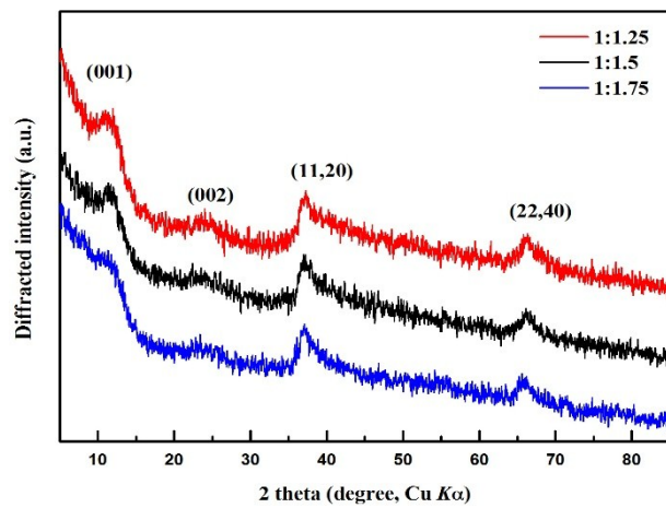
Fig. S1 the Power XRD patterns of Bir-H 2 O 2 samples with the molar ratio of KMnO 4 and H 2 O 2 at 1:1.25, 1:1.50, and 1:1.75.
