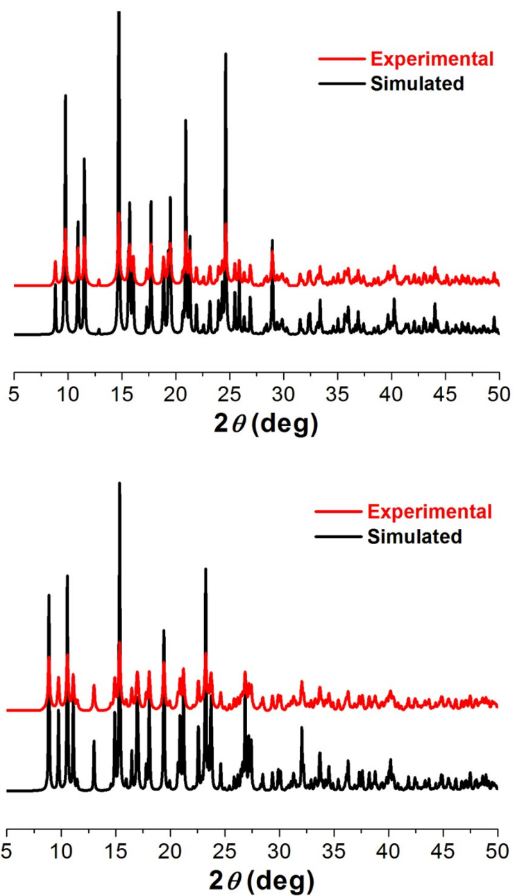
Fig. S1. PXRD patterns of complexes 1-2.
