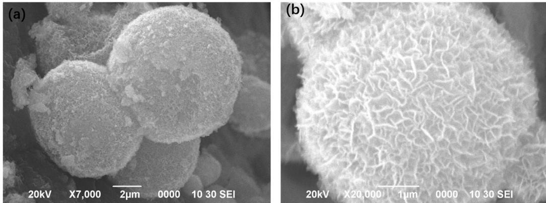
Fig. S1 SEM images of NiO nanoflowers.
