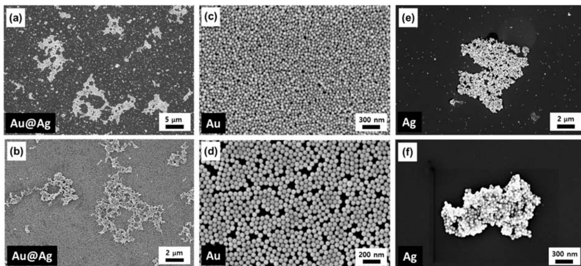
Fig. S1 SEM images of (a) and (b) Au@AgNCs, (c) and (d) AuNPs, (e) and (f) AgNPs on FTO after complete solvent evaporation.
