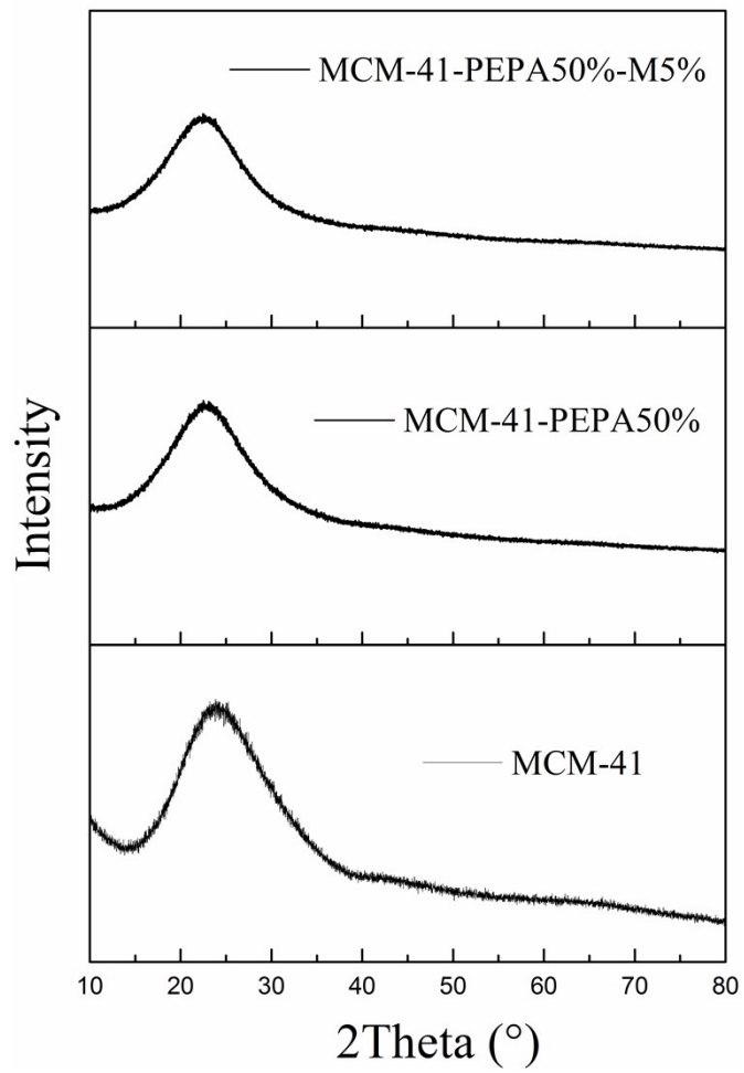
Fig.2S The XRD patterns for MCM-41 before and after PEPA and MPEG codispersion.
