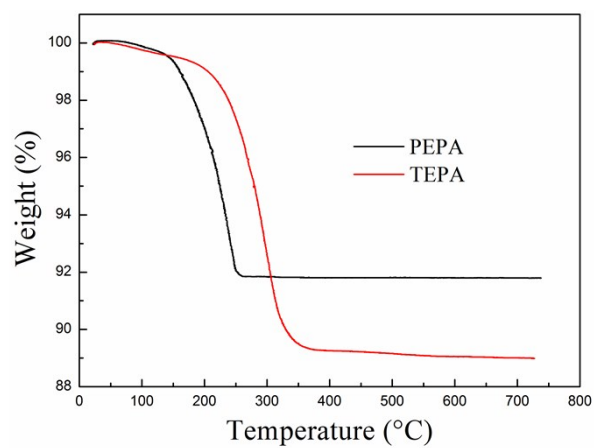
Fig.1S The thermal gravimetric curves for PEPA and TEPA.
