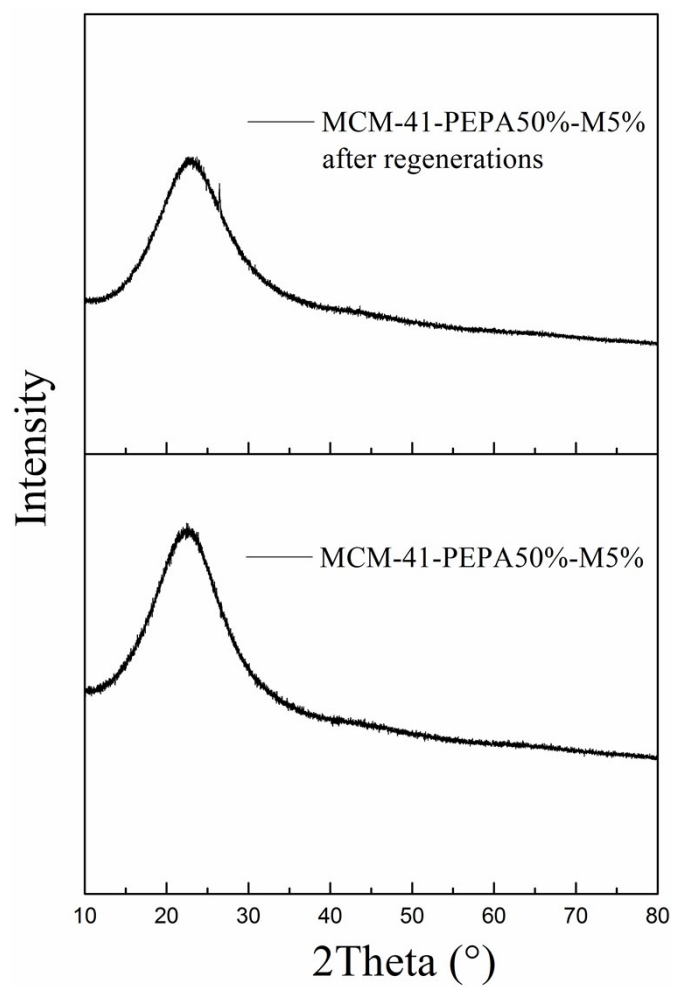
Fig.4S The XRD patterns for MCM-41-PEPA50%-M5% before and after 10 cycles.
