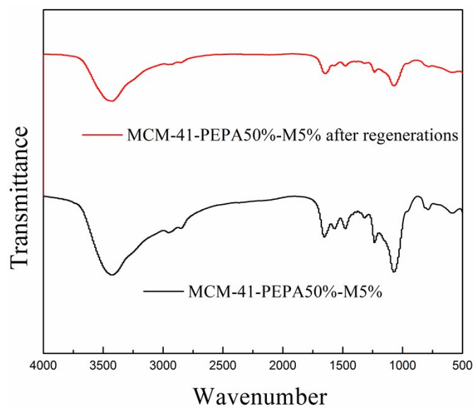
Fig.3S The FT-IR spectra for MCM-41-PEPA50%-M5% before and after 10 cycles.
