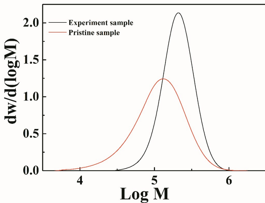
Fig. S3 Molecular weight distribution of pristine sample and experiment sample (SEC-RI).
