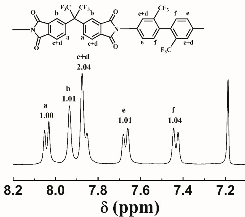
Fig. S2 ^1\text{H-NMR} spectra of 6FDA-TFDB PI sample.
