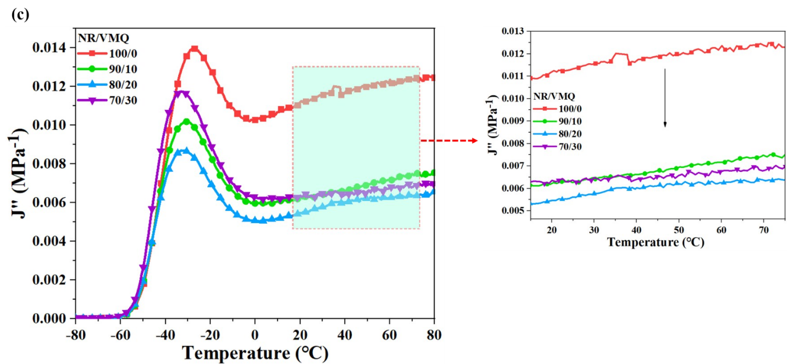
Fig. S1 Temperature dependency of viscoelastic parameters of NR/VMQ composites by DMTA: (a) Storage modulus E' , (b) Loss factor \tan \delta , (c) Loss compliance modulus J''
