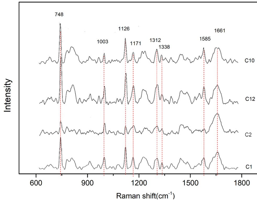
Fig. S1 Raman spectra of strains C1, C2, C10, C12.
