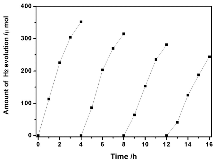
Figure S1. The cycle test of photocatalytic H 2 evolution of Ni@NiO/CdS photocatalyst.
