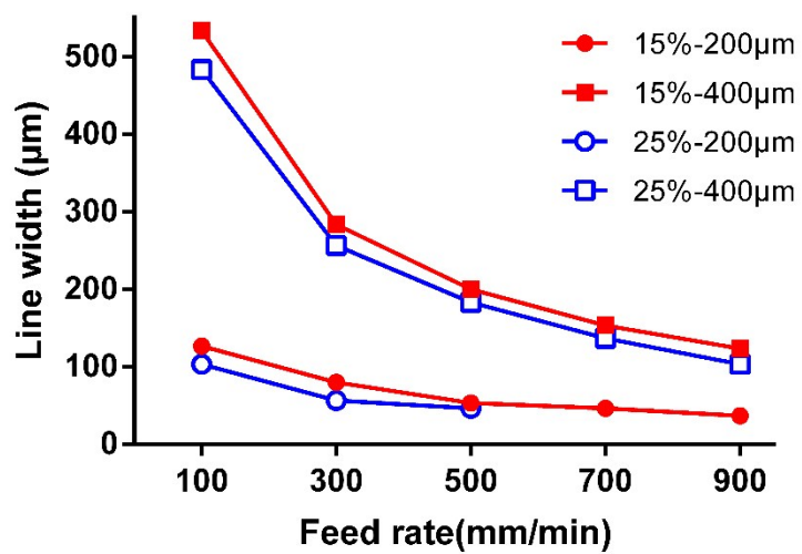
Fig S 2. Printing line width of the contrast powder mixed PCL (concentration – nozzle diameter)
