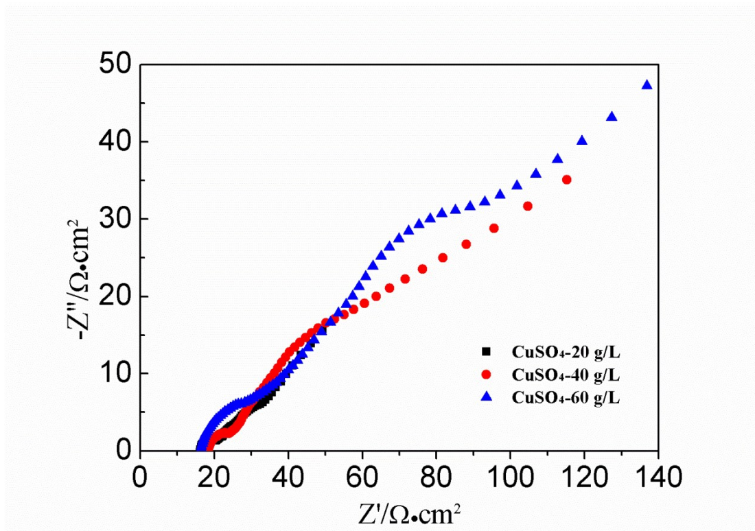
Figure S3 EIS curves of the \text{CuSO}_4/\text{DMF}/\text{H}_2\text{O} with \text{CuSO}_4 content of 20 g/L, 40 g/L and 60 g/L
