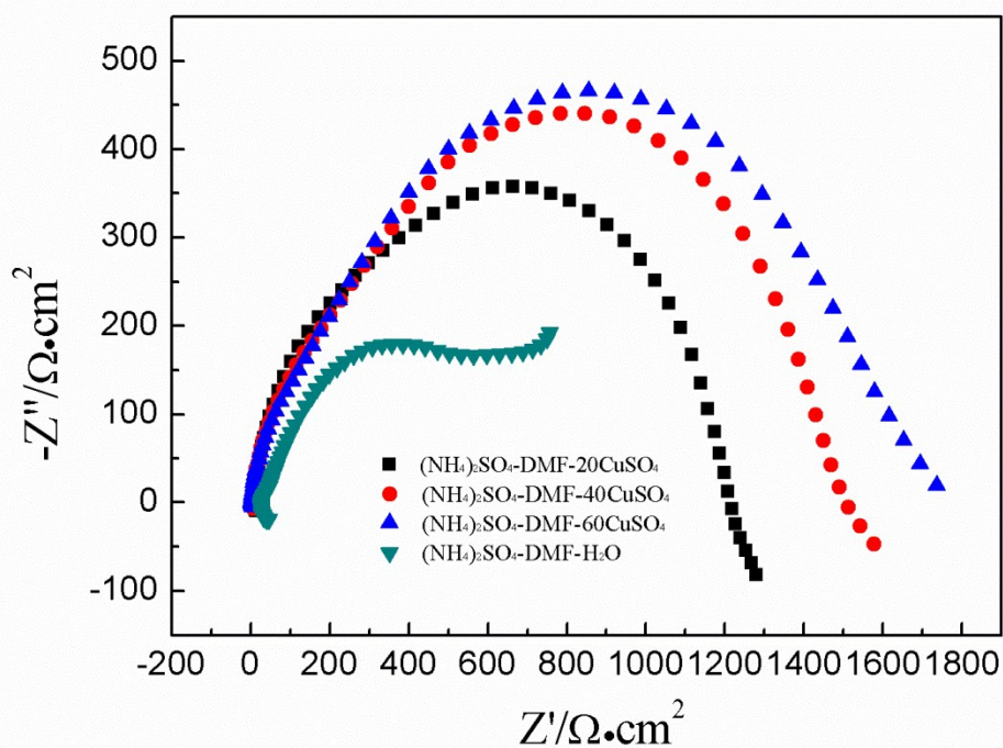
Figure S2 EIS curves of the (\text{NH}_4)_2\text{SO}_4/\text{DMF}/\text{H}_2\text{O} with and without \text{CuSO}_4
