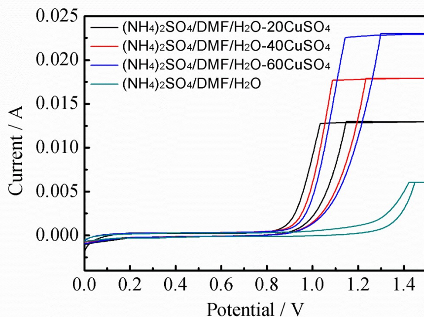
Figure S1 CV curves measured in the (\text{NH}_4)_2\text{SO}_4/\text{DMF}/\text{H}_2\text{O} solution and (\text{NH}_4)_2\text{SO}_4/\text{DMF}/\text{H}_2\text{O} solutions with different content of \text{CuSO}_4
