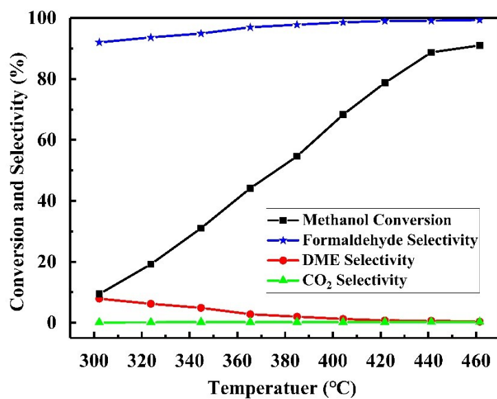
Fig. S2. The activity and selectivity test of \text{MoO}_3 .
