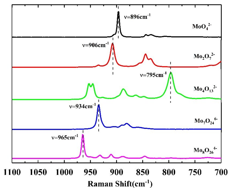
Fig. S1. Raman spectra of different pure solid isopolymolybdates.
