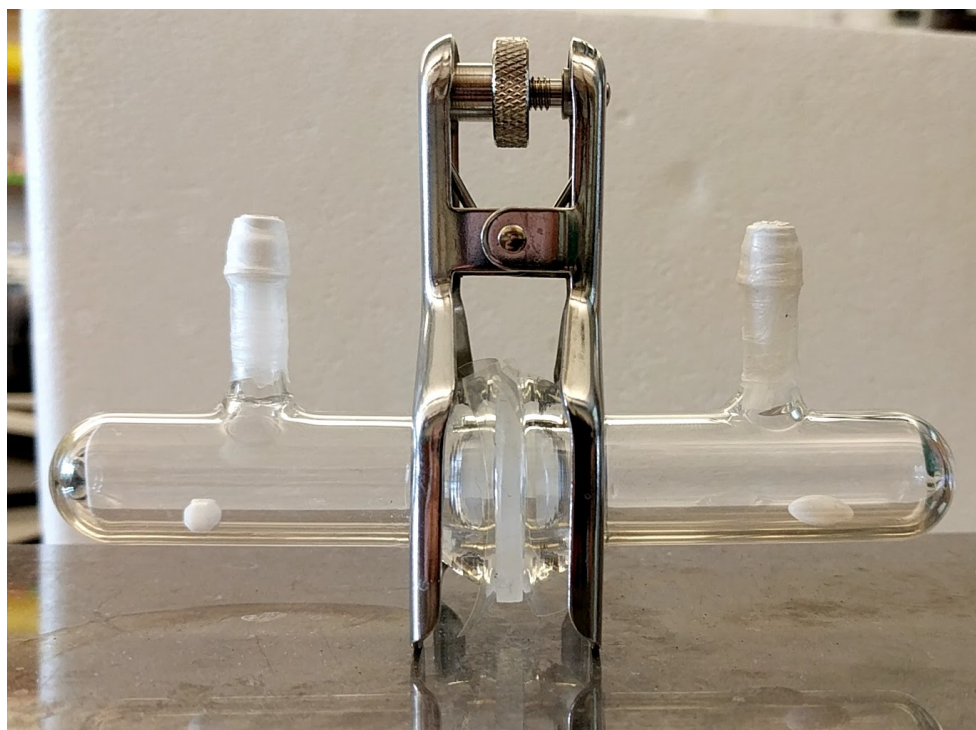
Figure S1. Picture of the assembled side-by-side glass diffusion cell.
