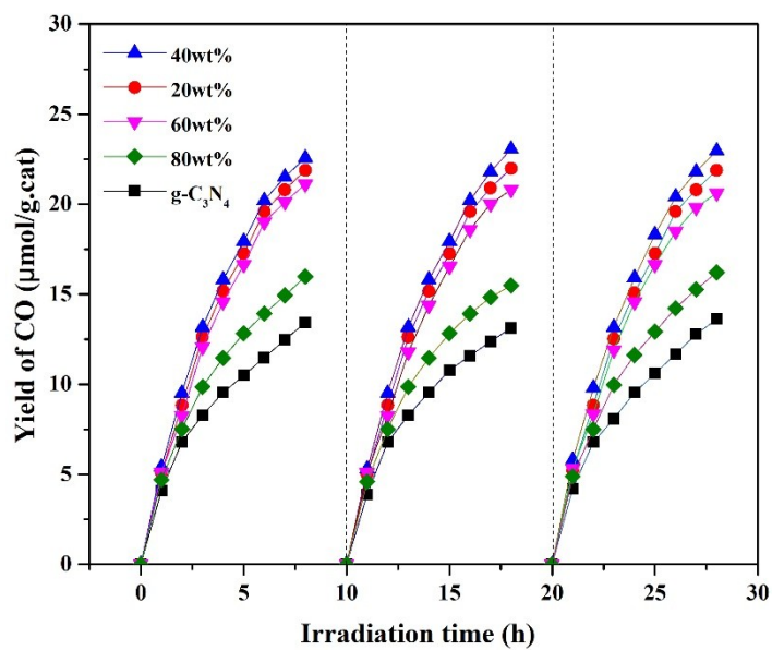
Fig. S1 Cycle characteristic diagram for all composites and pure g-C 3 N 4 .
