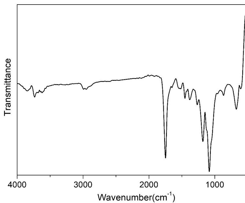
Supplementary Figure 1. FTIR spectrum of drug-free PLGA microspheres
