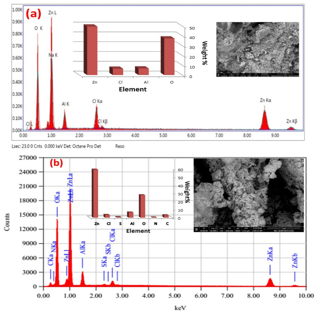
Fig S1: EDX of (a) Zn-Al LDH, (b) Zn-Al LDH/Cefotax.
