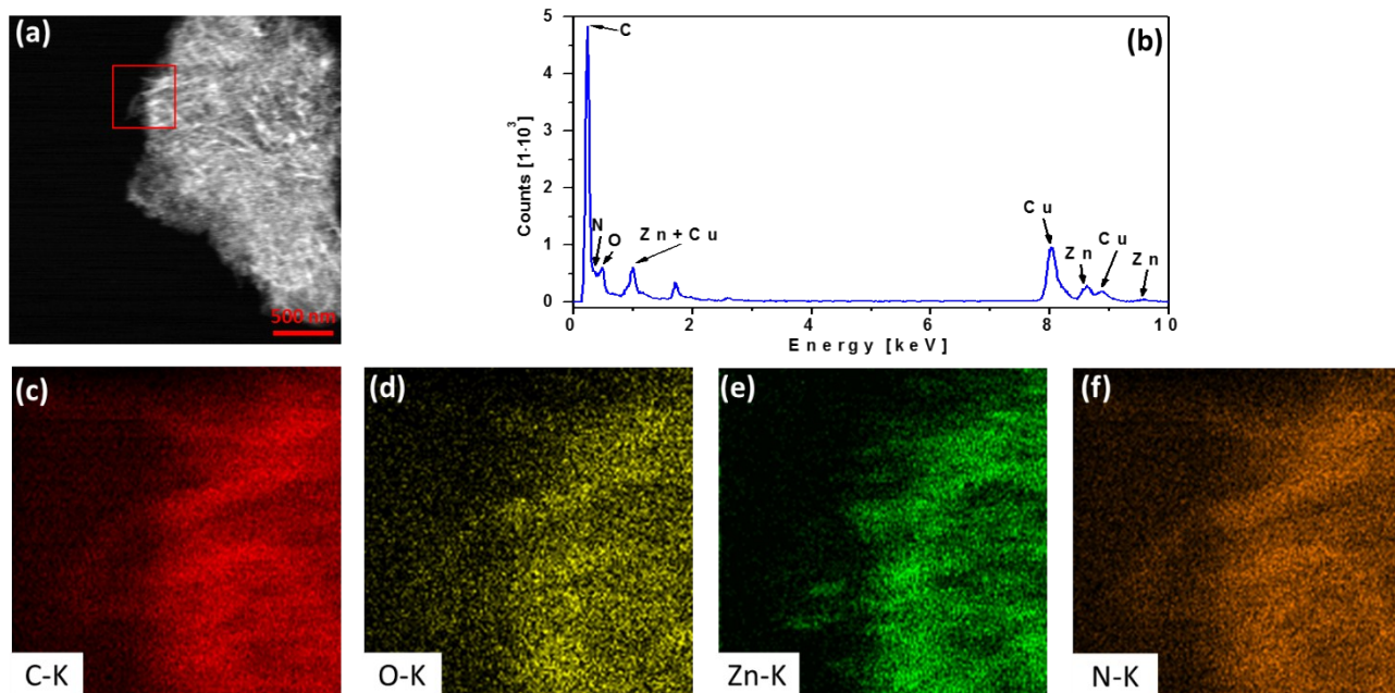
Figure S4. STEM image (a), EDX spectrum (b) and elemental mapping (c-f) of CMOF700-gCN.
