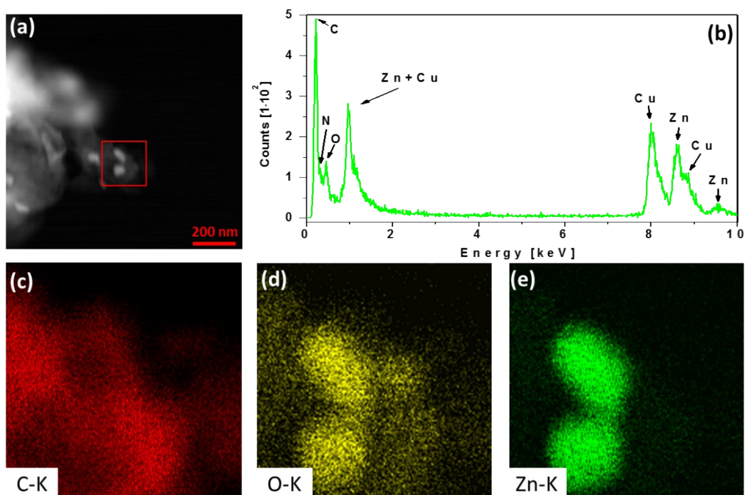
Figure S3. STEM image (a), EDX spectrum (b) and elemental mapping (c-e) of CMOF700.
