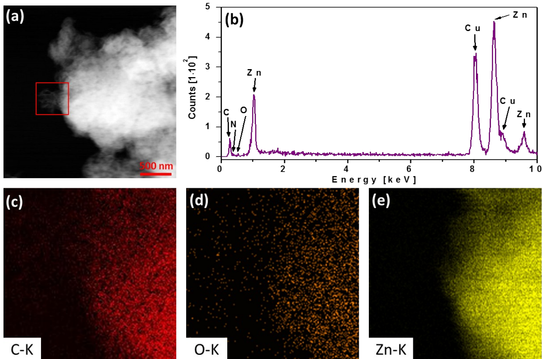
Figure S2. STEM image (a), EDX spectrum (b) and elemental mapping (c-e) of MOF5-gCN.
