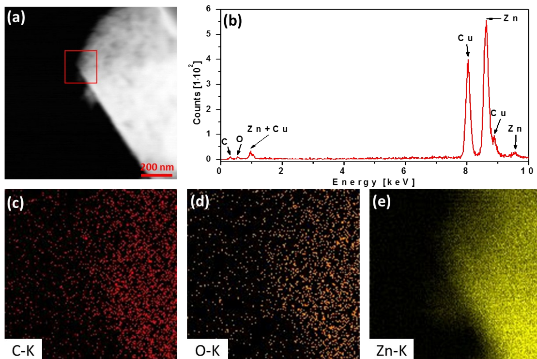
Figure S1. STEM image (a), EDX spectrum (b) and elemental mapping (c-e) of MOF5.
