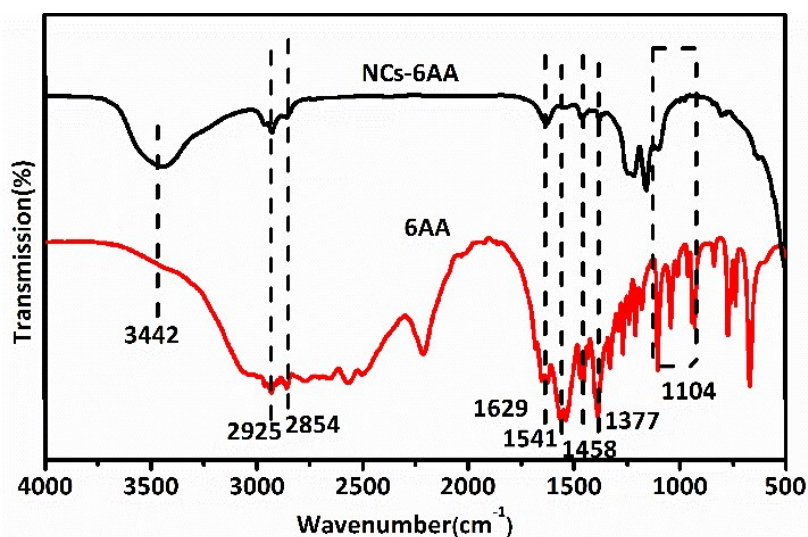
Fig. S1 FT-IR spectra of NCs modified with 6AA and pure 6AA.
