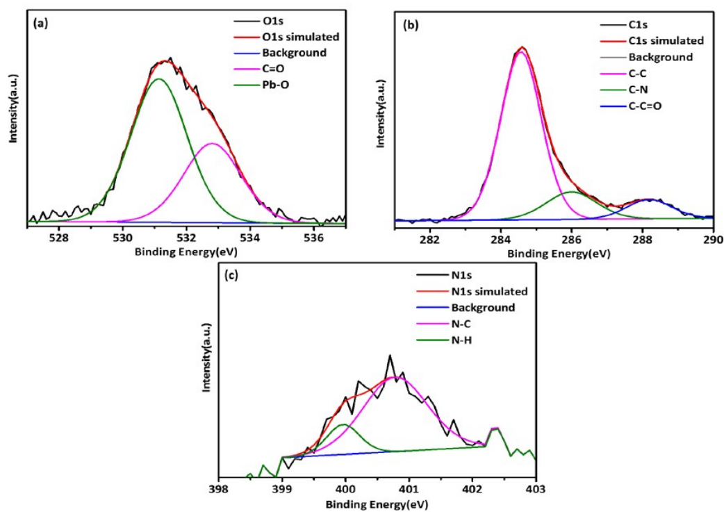
Fig. S2 High-resolution (a)O1s, (b) C1s, and (c) N1s XPS spectra of NCs modified with 6AA.
