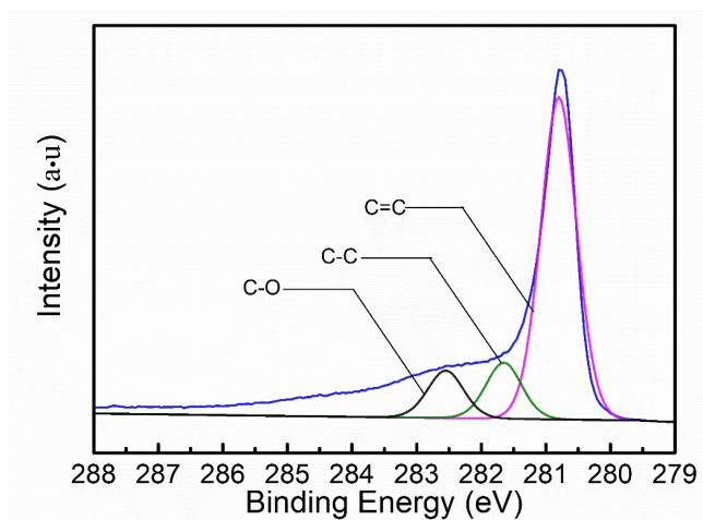
Figure S3 Corresponding C1s XPS spectra of graphene.
