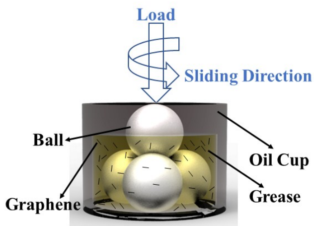
Figure S2 Schematic illustration of four-ball testing model.
