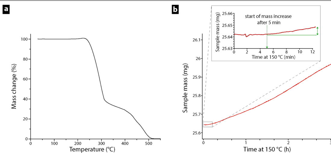
Fig. S2. Thermogravimetric measurements of LDPE without added antioxidants in an oxygen atmosphere with a temperature increase of 10\text{ °C min}^{-1} (a) and isothermal at 150\text{ °C} (b).
