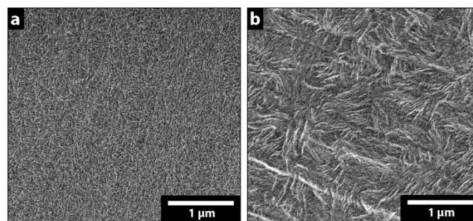
Fig. S3. Surface morphology of pressed thin film samples for using PET (a) and Al foil (b) as protective pressing films, respectively.
