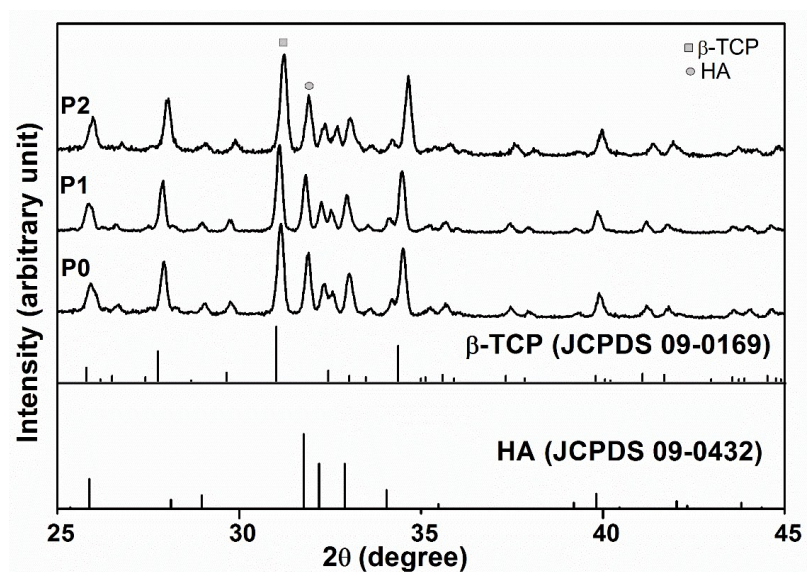
Supplementary Fig. S1 XRD patterns of various scaffolds
