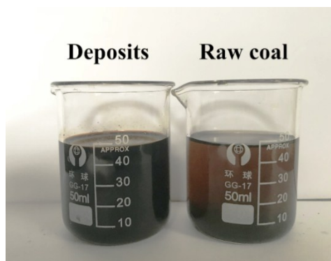
Fig. S2. Images of Deposit and raw coal dissolved in DMF after 48h
