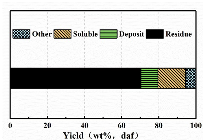
Fig. S1. The yield distribution of extraction products
