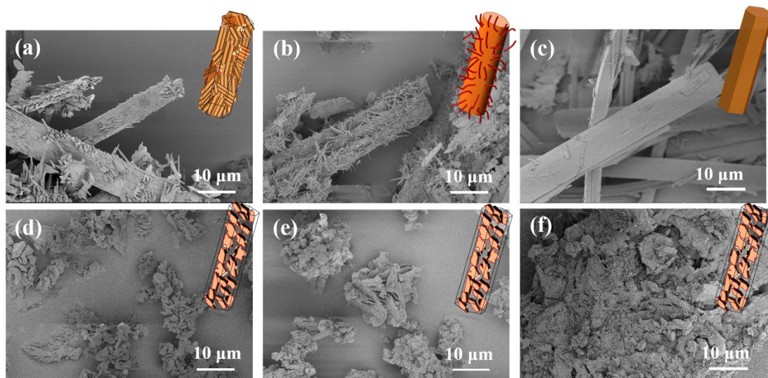
Figure S5 SEM images of the corroded M·2B 7 fibers by EA and EG for 1 minute: (a) M·2B 150 , (b) M·2B 200 (c) M·2B 400 after immersed in ethanol (EA); (d) M·2B 150 , (e) M·2B 200 , (f) M·2B 400 after immersed in ethylene glycol (EG). The insets are the corresponding diagram illustration.
