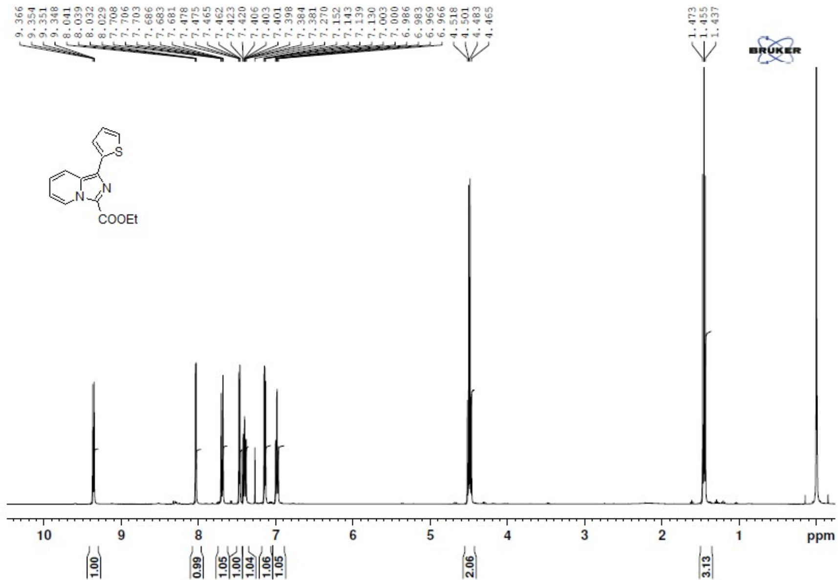
5) 1 H NMR spectra of Ethyl 1-(2-thionyl)imidazo[1,5-a]pyridine-3-carboxylate (3c)
