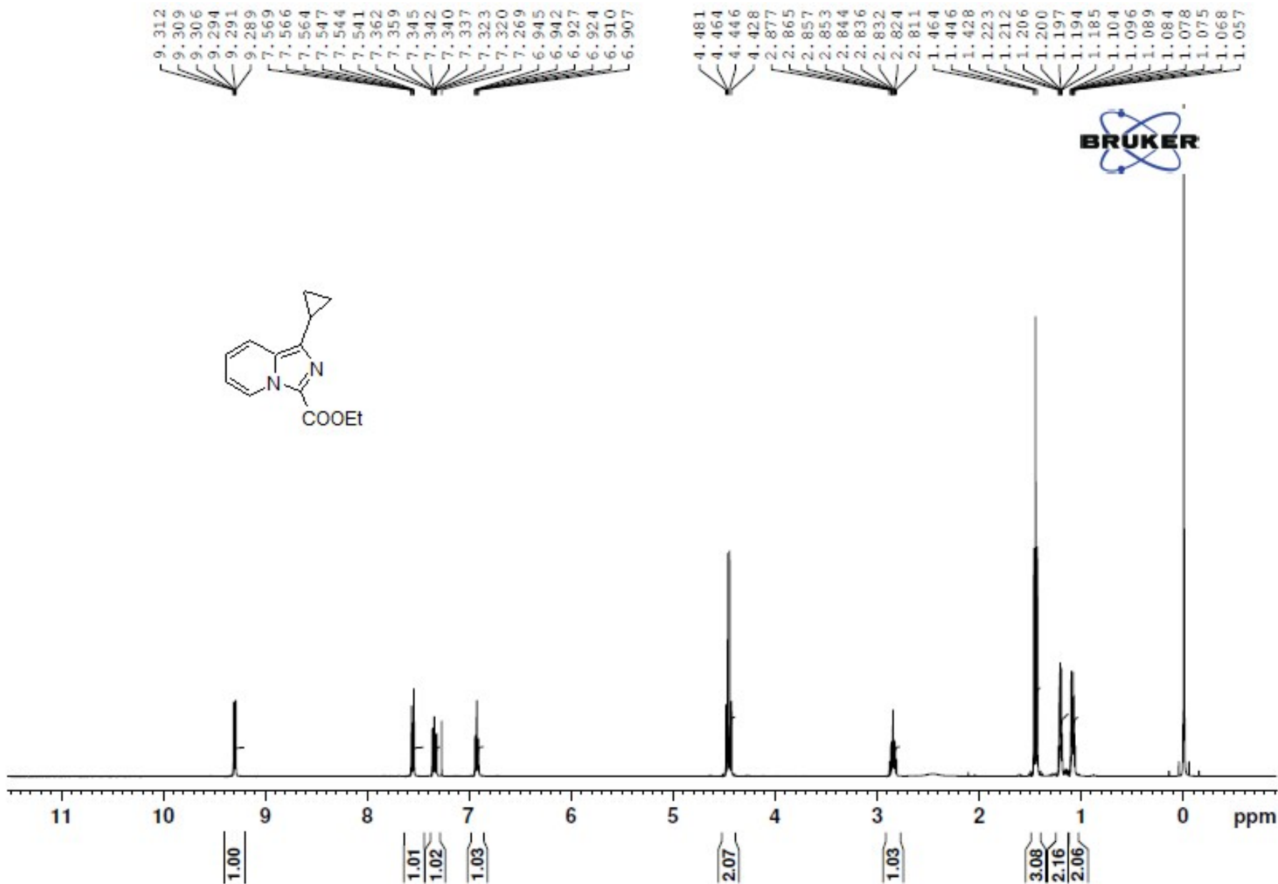
13) 1 H NMR spectra of Ethyl 1-cyclopropylimidazo[1,5-a]pyridine-3-carboxylate (3g)
