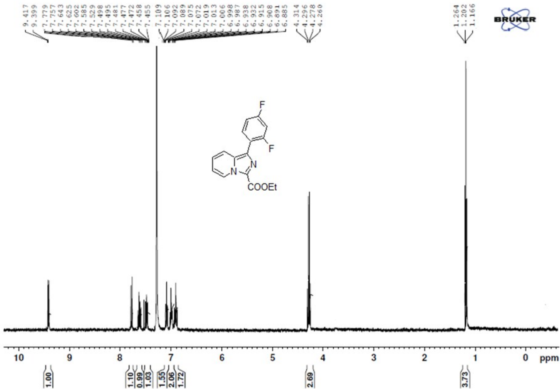
21) 1 H NMR spectra of Ethyl 1-(2,4-difluorophenyl)imidazo[1,5-a]pyridine-3-carboxylate (3k)
