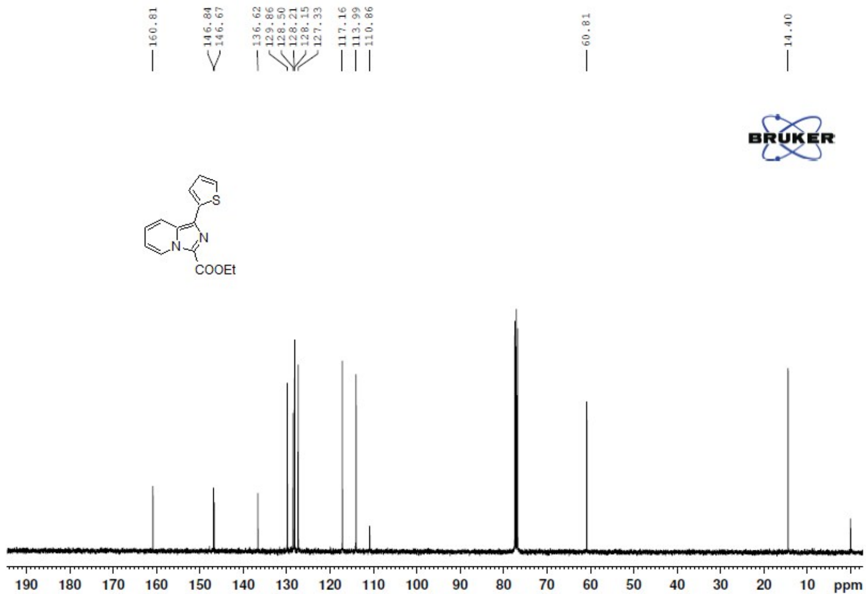
6) 13 C NMR spectra of Ethyl 1-(2-thionyl)imidazo[1,5-a]pyridine-3-carboxylate (3c)
