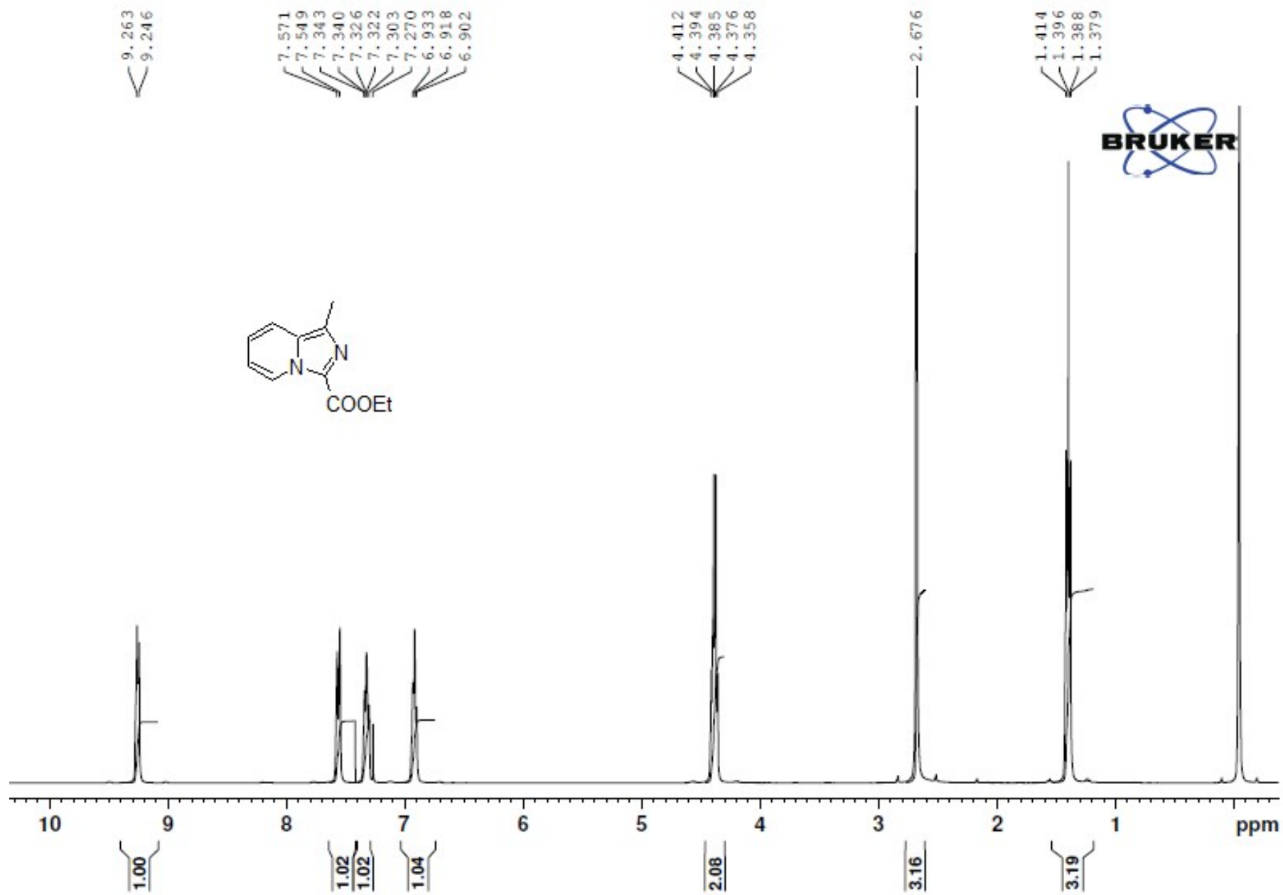
9) 1 H NMR spectra of Ethyl 1-methylimidazo[1,5-a]pyridine-3-carboxylate (3e)
