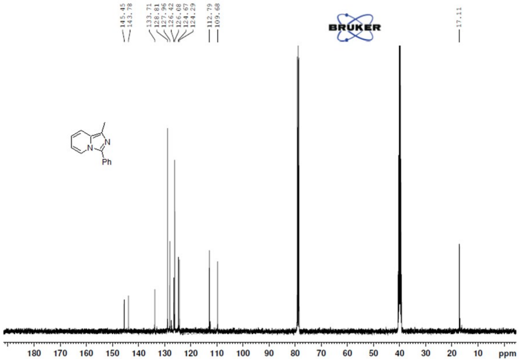
24) 13 C NMR spectra of 1-Methyl-3-phenylimidazo[1,5-a]pyridine (3m)
