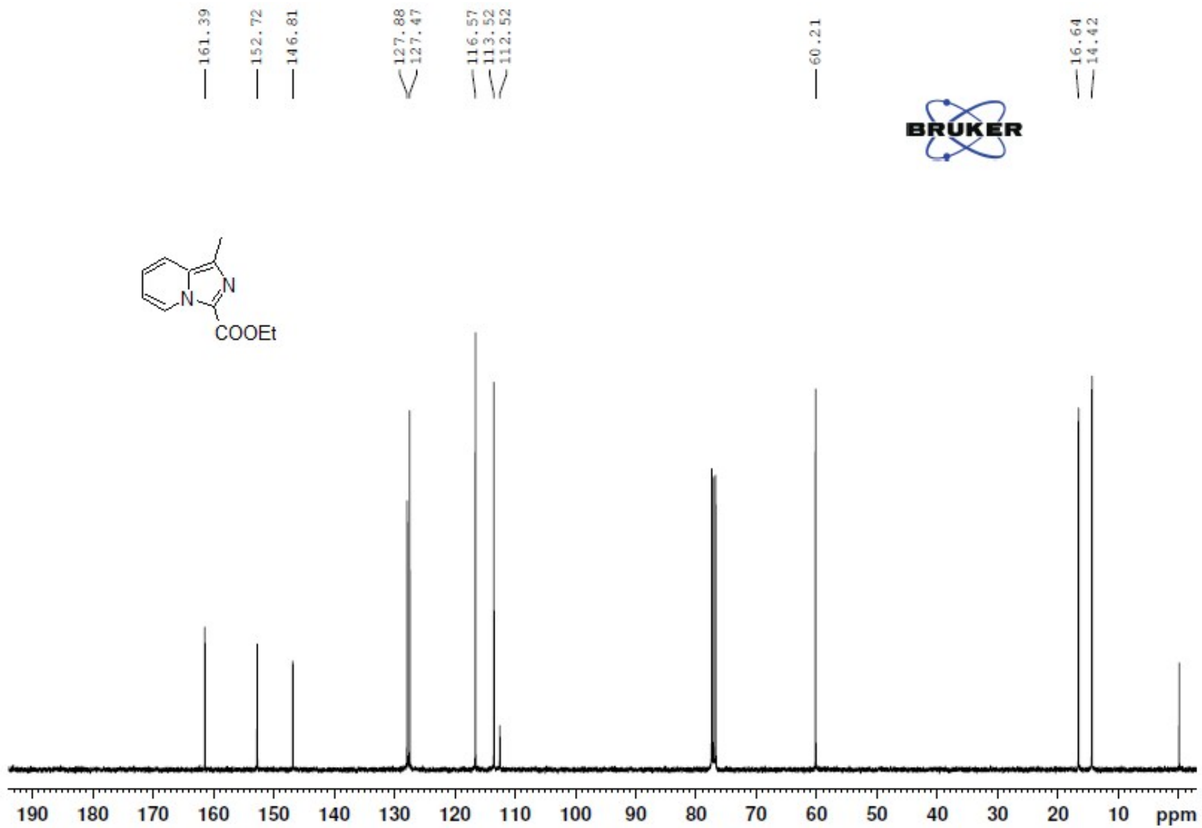
10) 13 C NMR spectra of Ethyl 1-methylimidazo[1,5-a]pyridine-3-carboxylate (3e)
