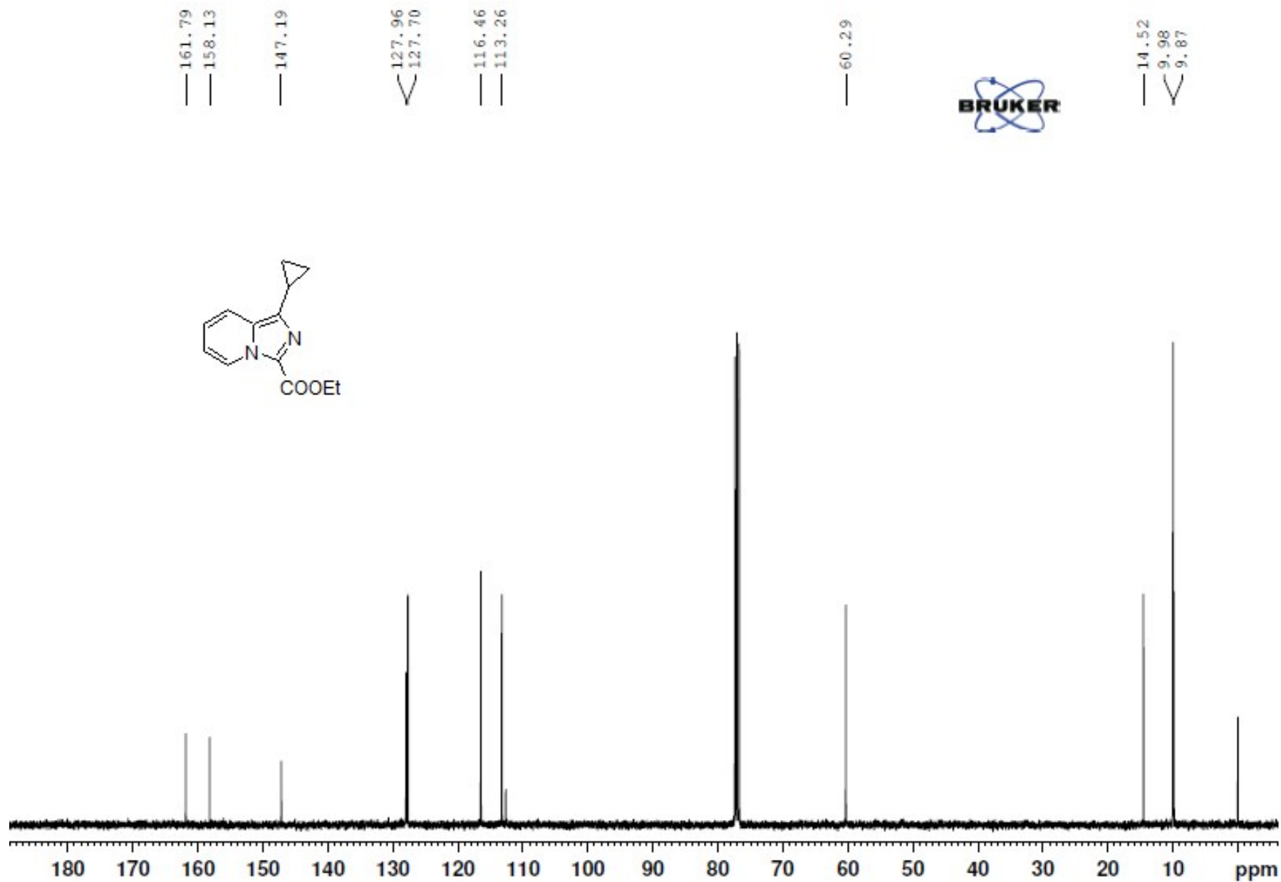
14) ^{13}\text{C} NMR spectra of Ethyl 1-cyclopropylimidazo[1,5-a]pyridine-3-carboxylate (3g)
