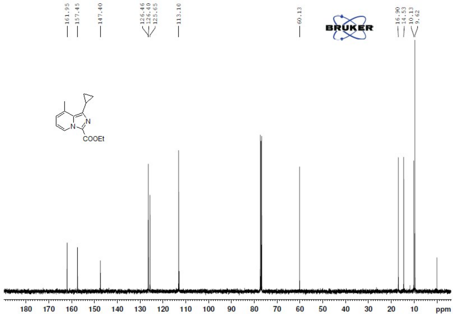
16) 13 C NMR spectra of Ethyl 1-cyclopropyl-8-methylimidazo[1,5-a]pyridine-3-carboxylate (3h)
