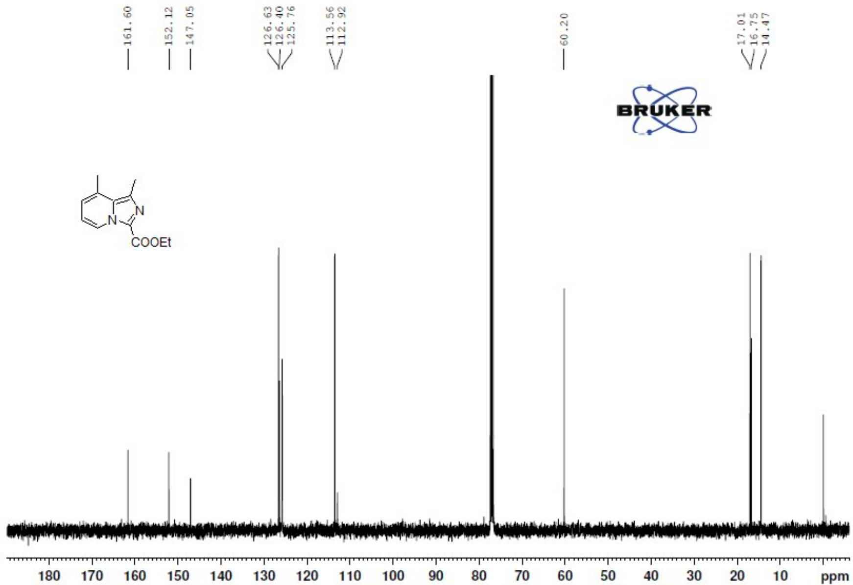
12) 13 C NMR spectra of Ethyl 1,8-dimethylimidazo[1,5-a]pyridine-3-carboxylate (3f)
