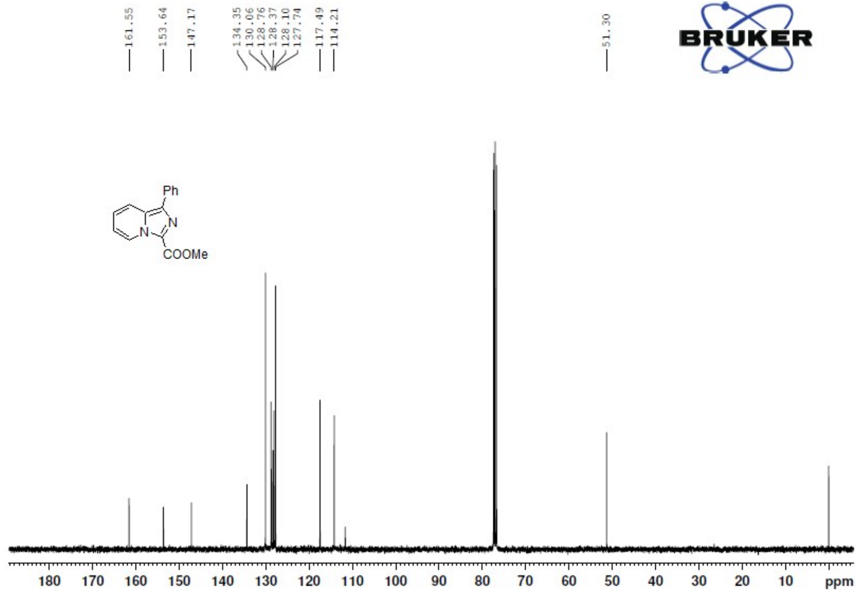
2) 13 C NMR spectra of Methyl 1-phenylimidazo[1,5-a]pyridine-3-carboxylate (3a)
