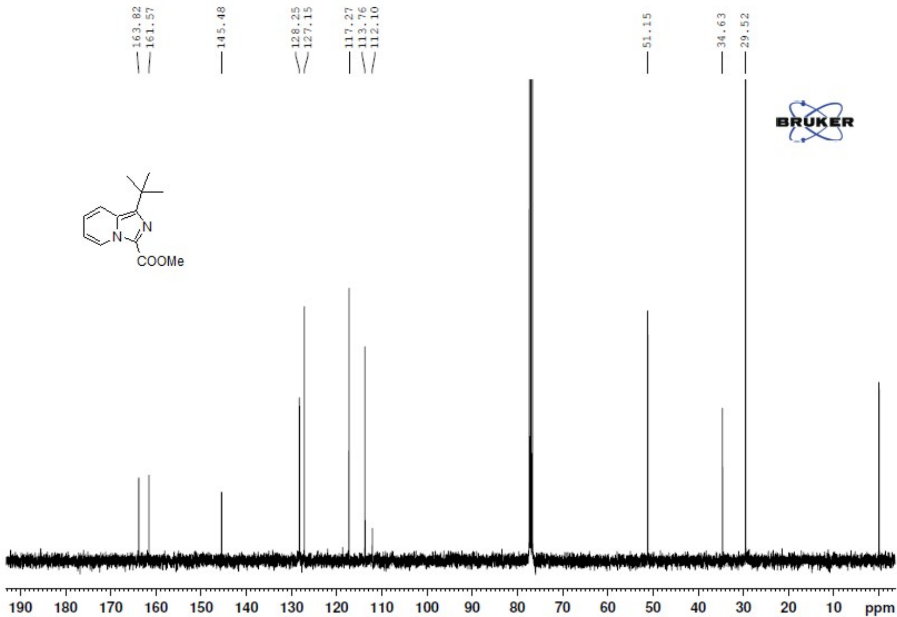
18) ^{13}\text{C} NMR spectra of Methyl 1-tert-butylimidazo[1,5-a]pyridine-3-carboxylate (3i)
