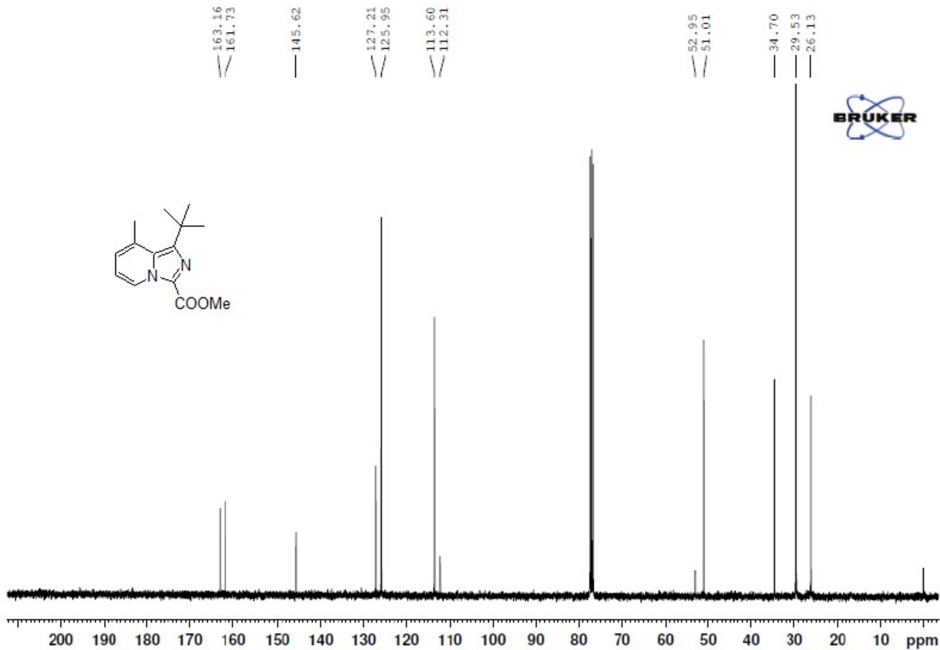
20) ^{13}\text{C} NMR spectra of Methyl 1-tert-butylimidazo[1,5-a]pyridine-3-carboxylate (3j)
