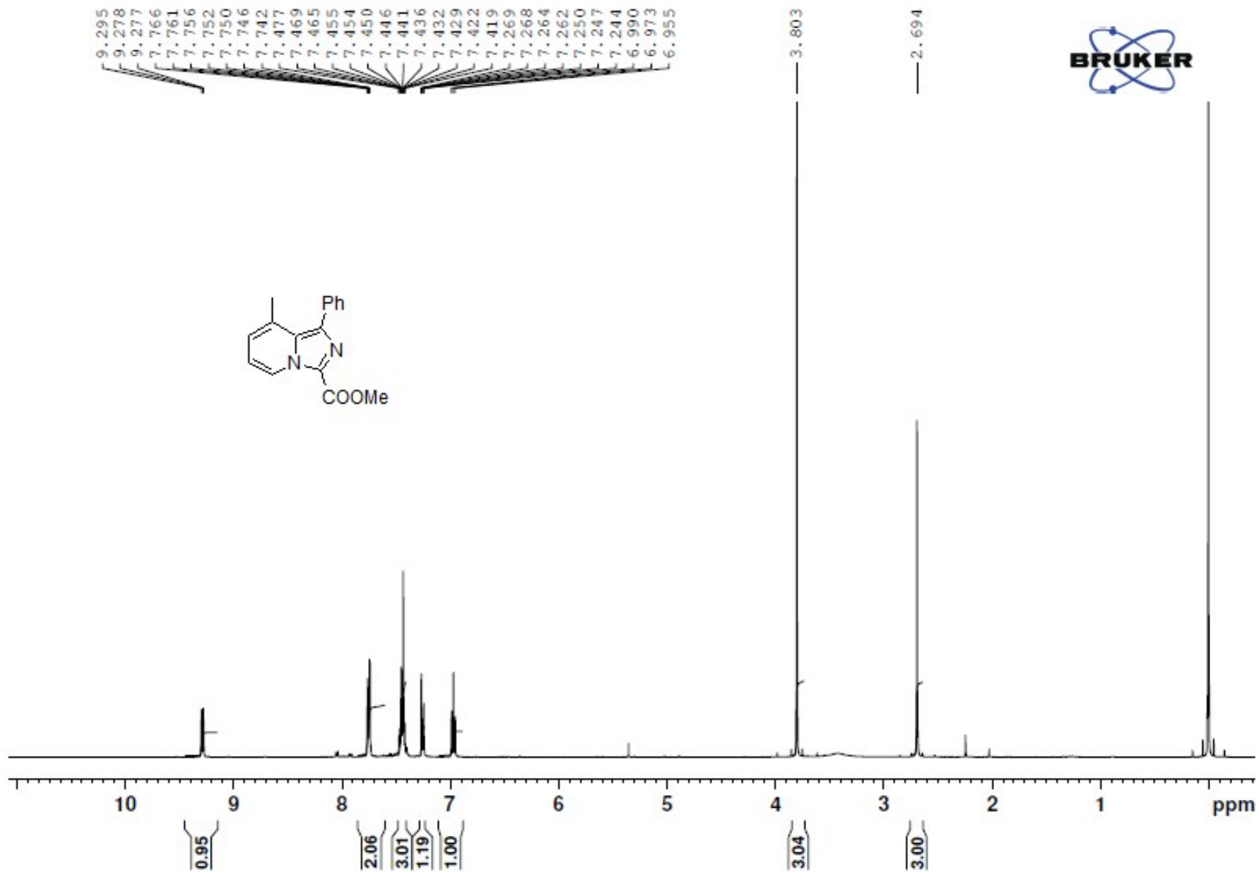
3) 1 H NMR spectra of Methyl 8-methyl-1-phenylimidazo[1,5-a]pyridine-3-carboxylate (3b)
