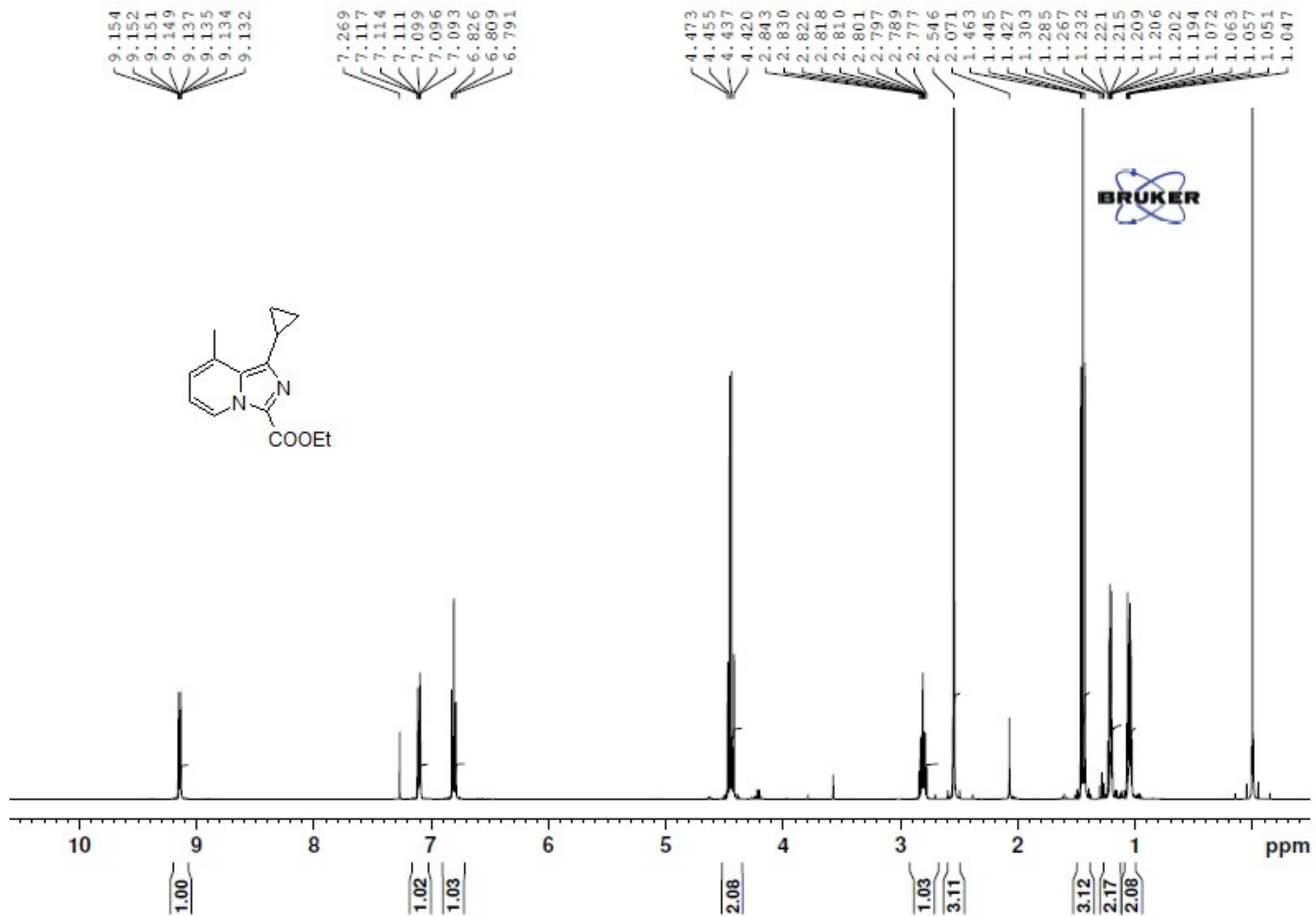
15) 1 H NMR spectra of Ethyl 1-cyclopropyl-8-methylimidazo[1,5-a]pyridine-3-carboxylate (3h)
