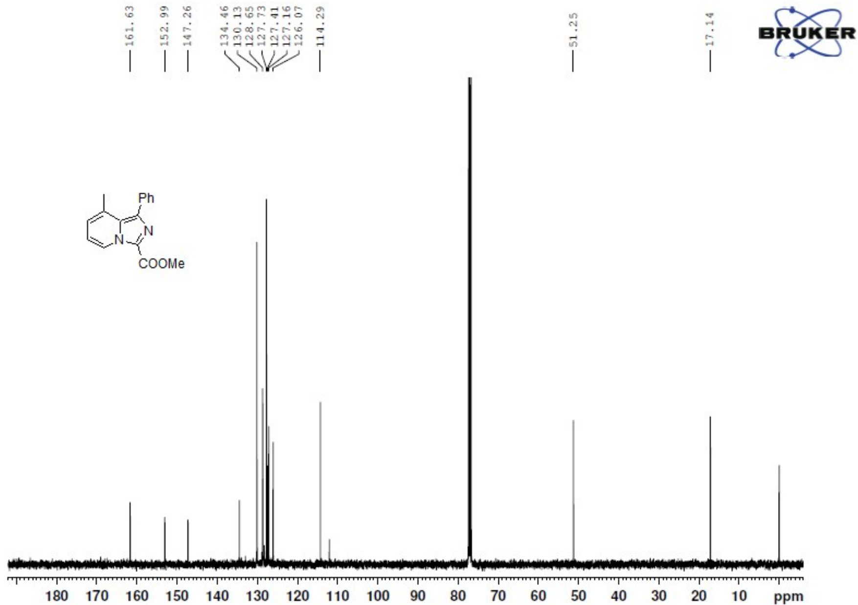
4) ^{13}\text{C} NMR spectra of Methyl 8-methyl-1-phenylimidazo[1,5-a]pyridine-3-carboxylate (3b)
