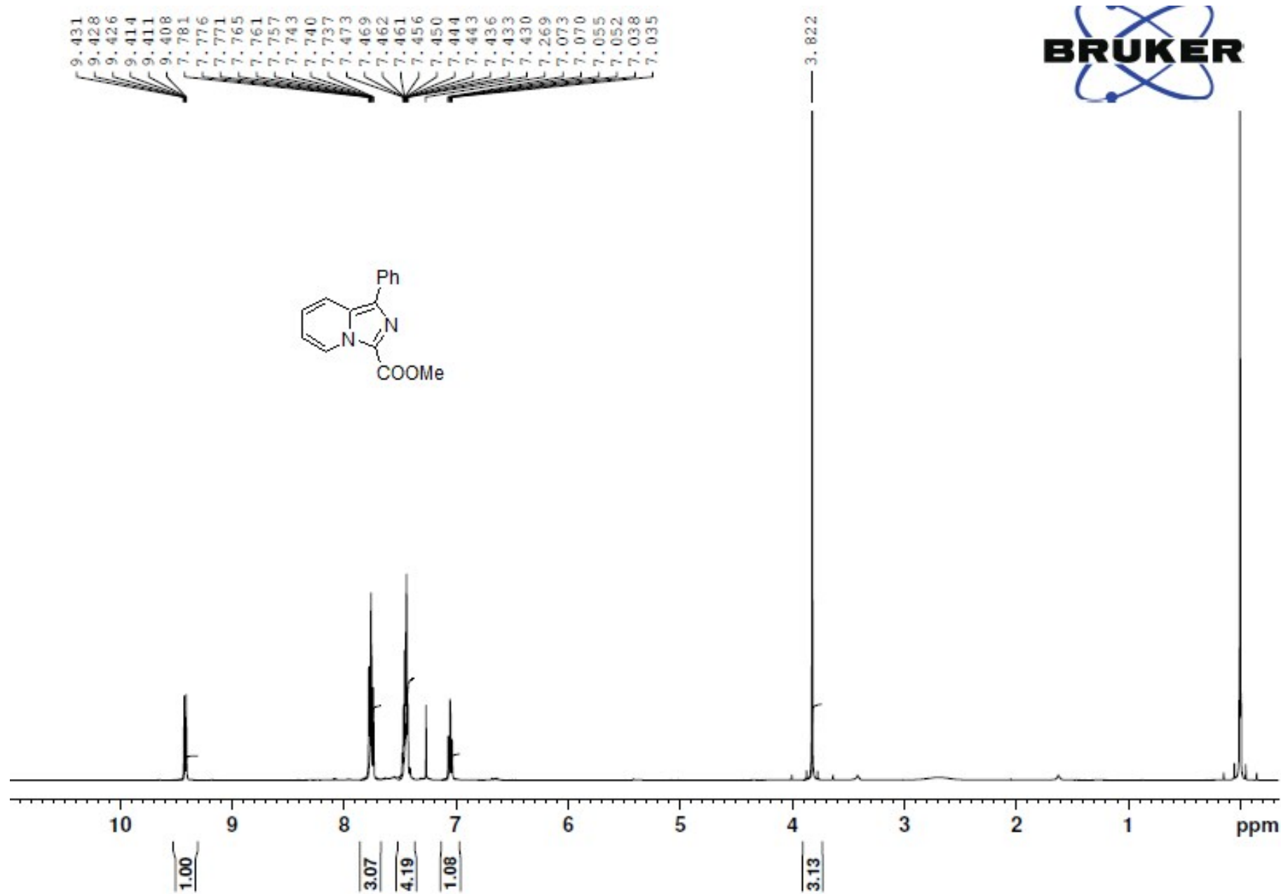
1) 1 H NMR spectra of Methyl 1-phenylimidazo[1,5-a]pyridine-3-carboxylate (3a)
