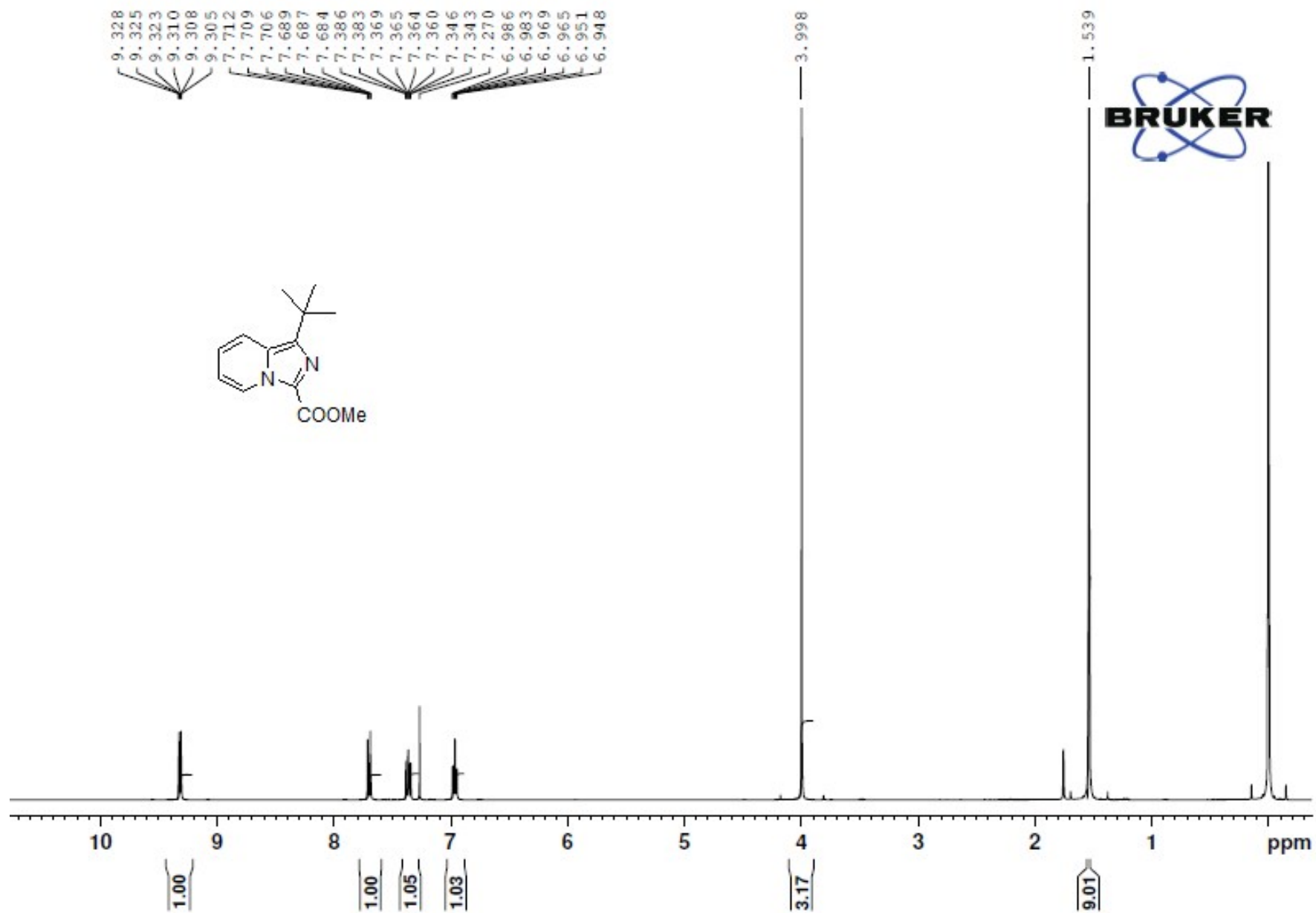
17) 1 H NMR spectra of Methyl 1-tert-butylimidazo[1,5-a]pyridine-3-carboxylate (3i)
