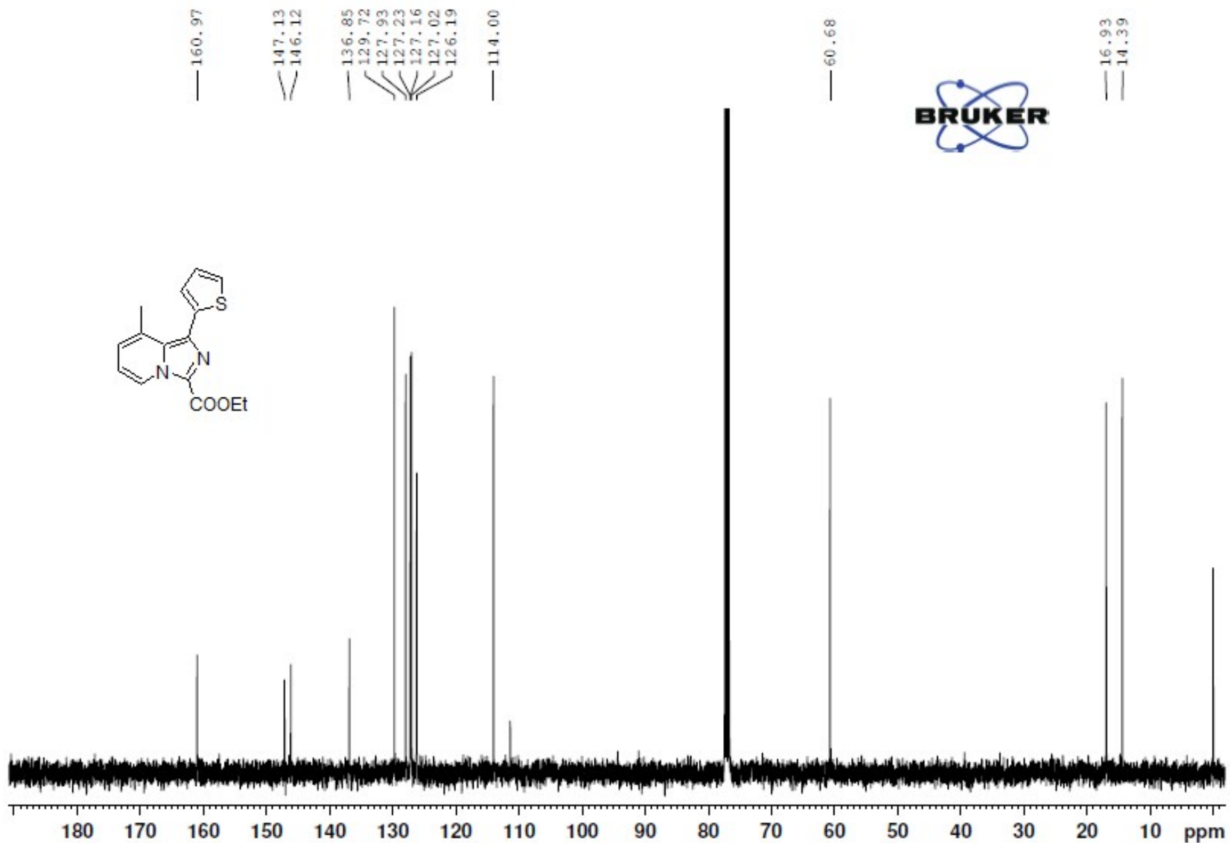
8) 13 C NMR spectra of Ethyl 1-(2-thionyl)-8-methylimidazo[1,5-a]pyridine-3-carboxylate (3d)
