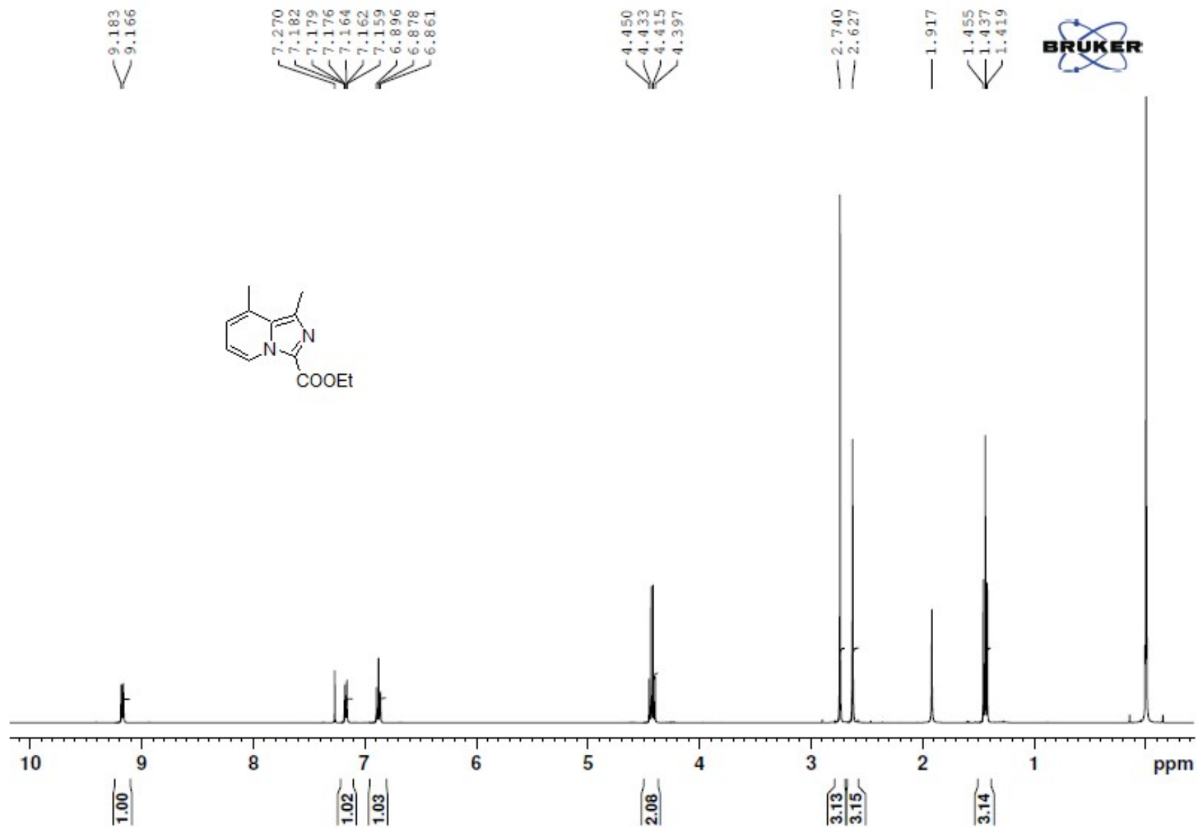
11) 1 H NMR spectra of Ethyl 1,8-dimethylimidazo[1,5-a]pyridine-3-carboxylate (3f)
