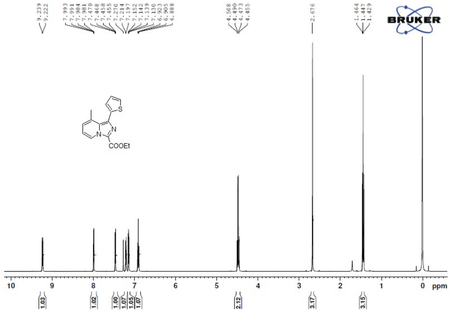
7) 1 H NMR spectra of Ethyl 1-(2-thionyl)-8-methylimidazo[1,5-a]pyridine-3-carboxylate (3d)
