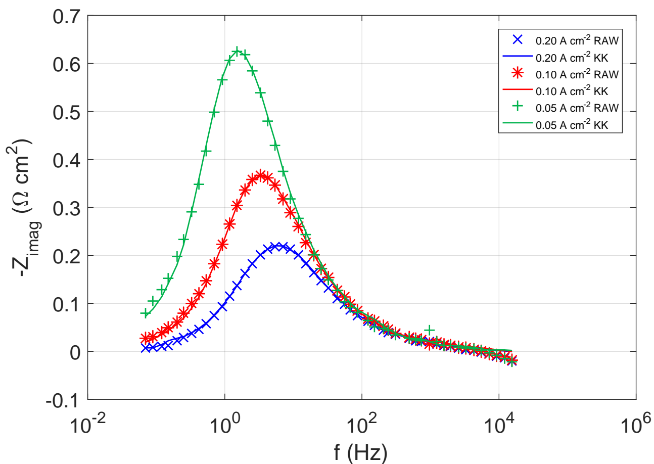
Figure S1. Example of imaginary part of spectra as measured (symbols) or simulated by Kramers-Kronig analysis. Sample with 1 \text{mg cm}^{-2} catalyst loading and 45% ionomer content.
