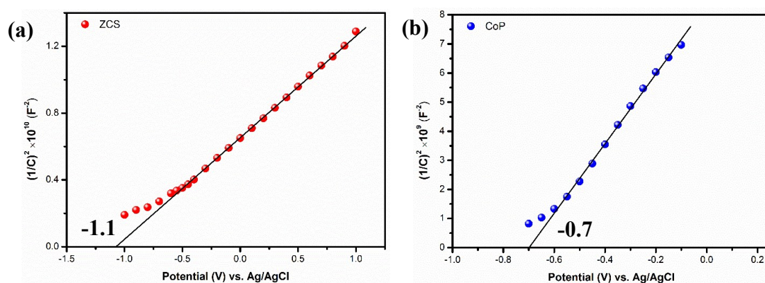
Fig. S4 Mott-Schottky plot of (a) ZCS (b) CoP.
