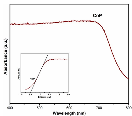
Fig. S3 UV-vis DRS spectra of CoP (Inset: Tauc plot of CoP).
