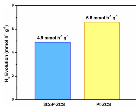
Fig. S2 Photocatalytic H 2 evolution activity comparison between 3CoP-ZCS and Pt-ZCS.
