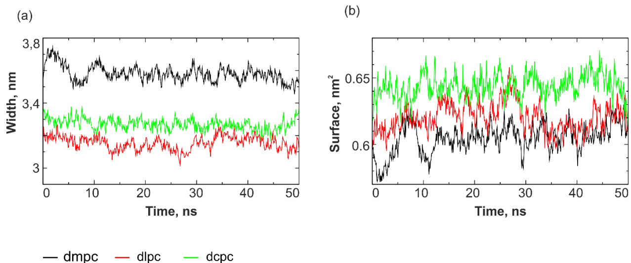
Figure S1 (a) Thickness and (b) area per lipid of bilayers formed by DLPC, diC12cp-PC, or DMPC in the course of MD simulations of systems containing 200 lipid molecules each with approximately 10000 water molecules added.
