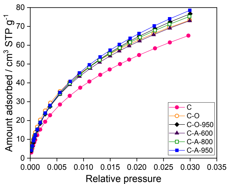
Figure S1. Carbon dioxide adsorption isotherms
