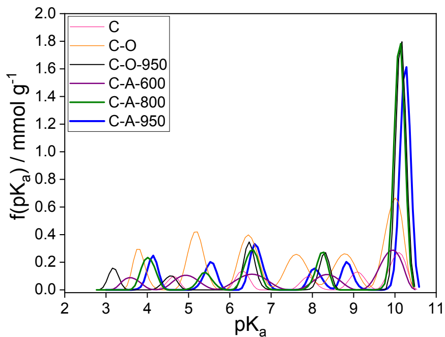
Figure S2. pK_a distributions.
