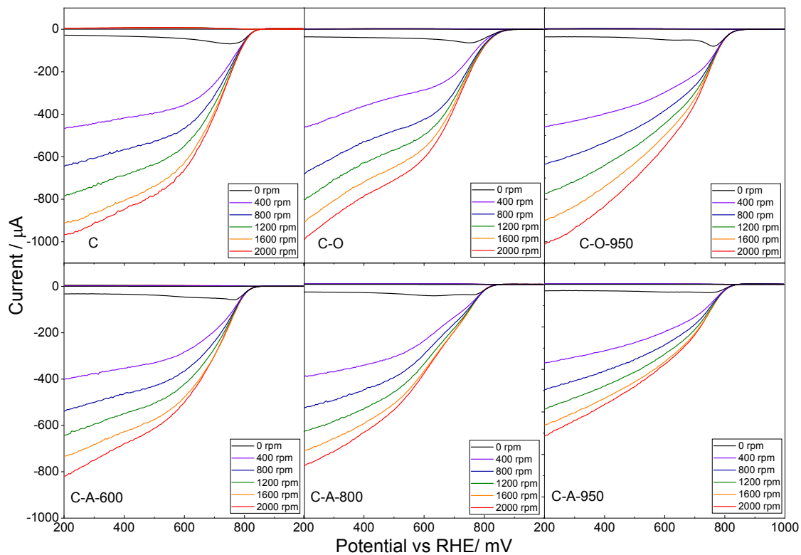
Figure S3. LSV curves of the modified and unmodified carbons.
