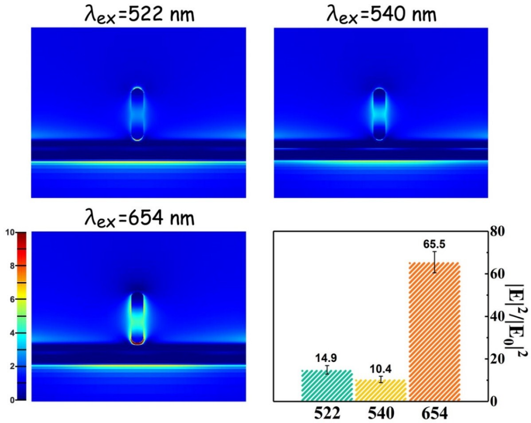
S8. Electric field distributions of simulation model of Au NRs/W 18 O 49 NWs (vertical contact model) under different light excitation.
