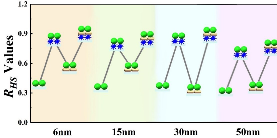
S7. R_{HS} values as a function of different grain size of NaYF 4 NPs in the NaYF 4 NPs, NaYF 4 NPs/W 18 O 49 NWs, NaYF 4 NPs/Au NRs, NaYF 4 NPs/Au NRs/W 18 O 49 NWs hybrid film.
