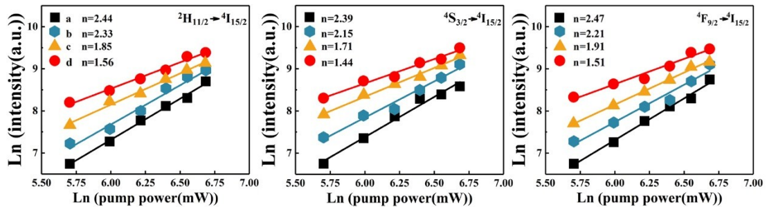
S6. Power density dependent UCL intensity of ^2H_{11/2} \rightarrow ^4I_{15/2} , ^4S_{3/2} \rightarrow ^4I_{15/2} , and ^4F_{9/2} \rightarrow ^4I_{15/2} transitions under 980 nm irradiation for a) NaYF 4 NPs, b) NaYF 4 NPs/W 18 O 49 NWs, c) NaYF 4 NPs/Au NRs, d) NaYF 4 NPs/Au NRs/W 18 O 49 NWs hybrid film.
