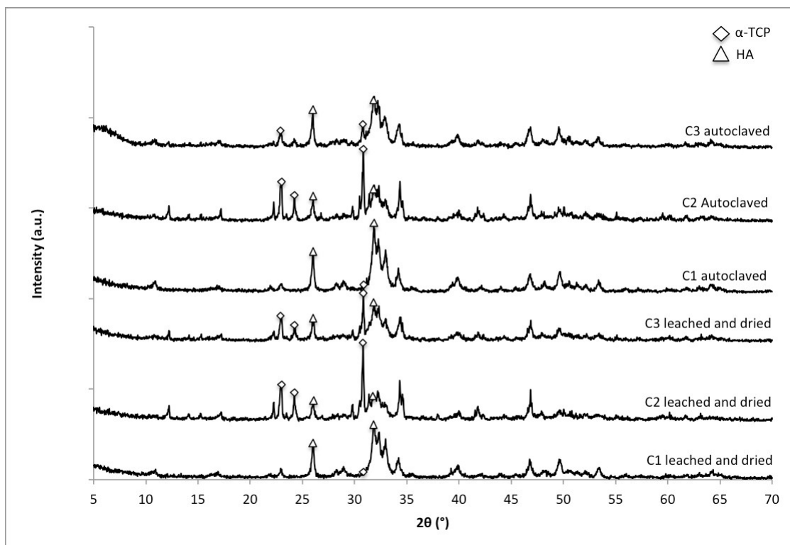
Figure S2 XRD patterns of Granule C: 3 bathes of dried and autoclaved
