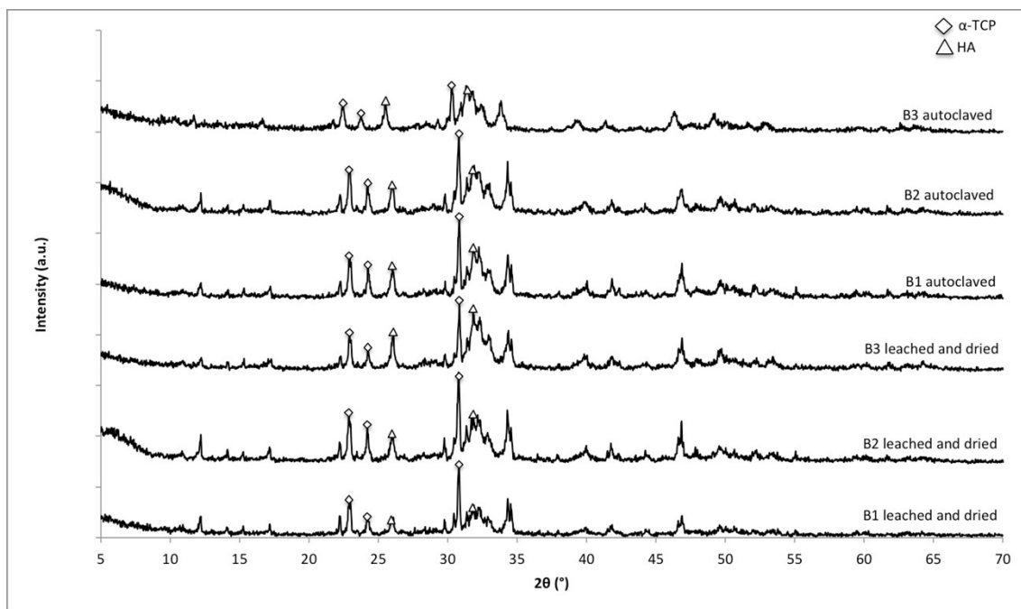
Figure S1 XRD patterns of Granule B: 3 bathes of dried and autoclaved
