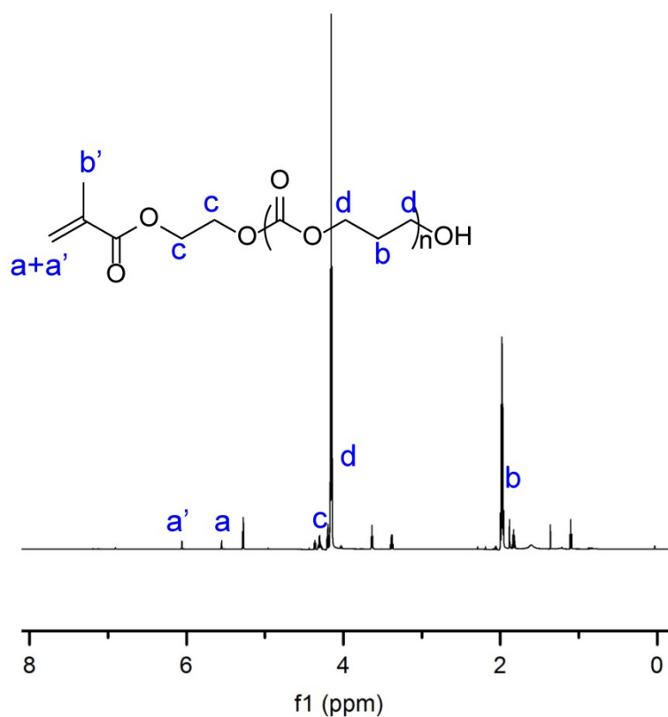
Figure S1. ^1\text{H} NMR spectra of HEMA-g-PTMC macromonomer in \text{CD}_2\text{Cl}_2 .
