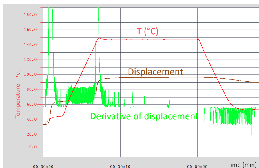
Figure SI 1: Evolution of SPS cursor displacement and its derivative for the example sample cACP
