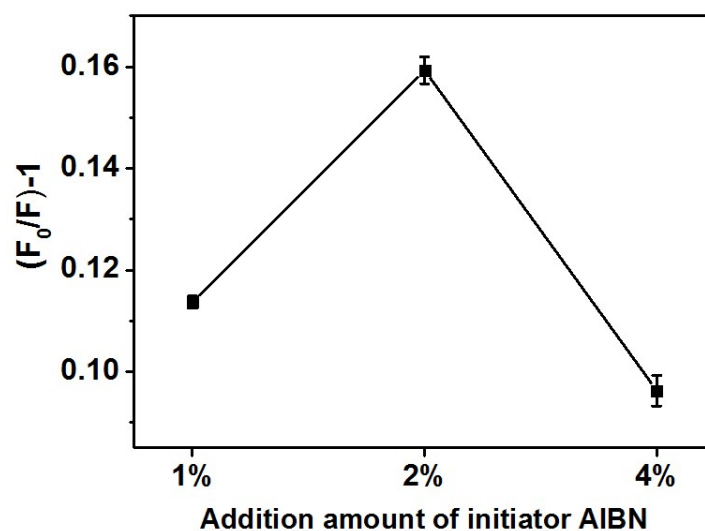
Figure S1. Effect of initiator addition amounts in the polymerization process of PBAN-GMA on the fluorescence response of B-FMIP NPs
