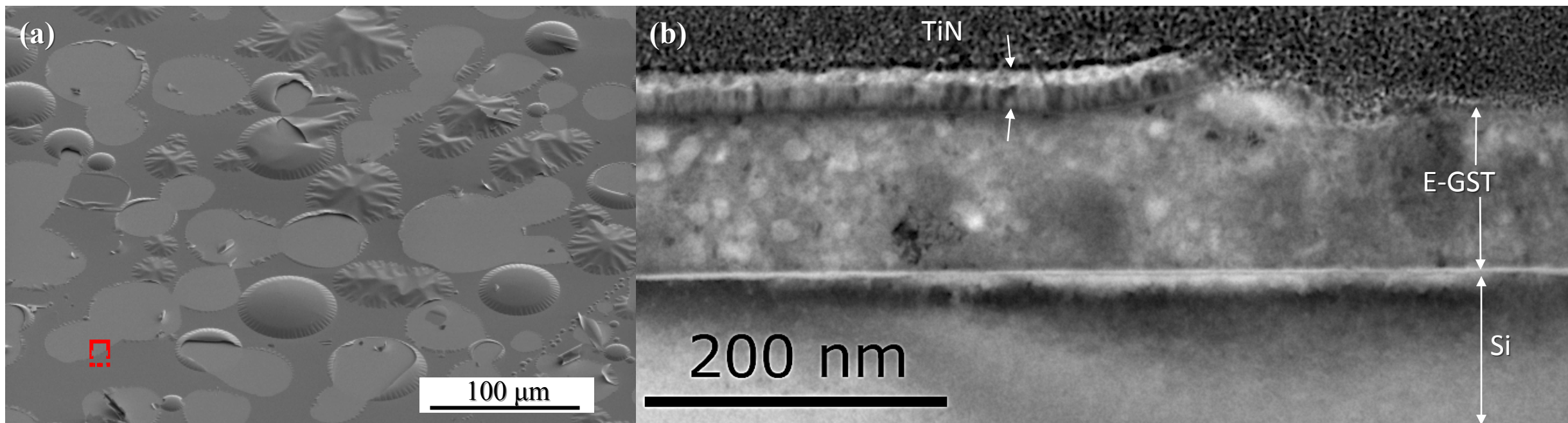
S1. (a) SEM image of the surface of E-GST annealed at 450°C for 30 minutes. (b) BT-TEM on FIB lamella cut in correspondence of a blister's edge, as shown by the red square in (a).
