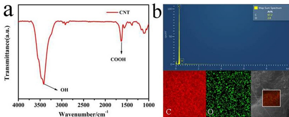
Fig S1. a) The FT-IR spectra of CNT, b) The EDS spectra of CNT.
