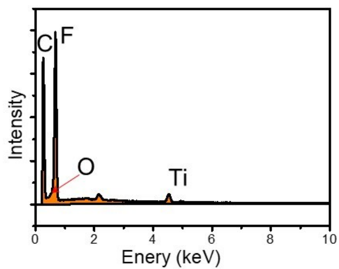
Fig. S2 The energy-dispersive X-ray spectroscopy (EDS) spectrum of MXene/PVDF film
