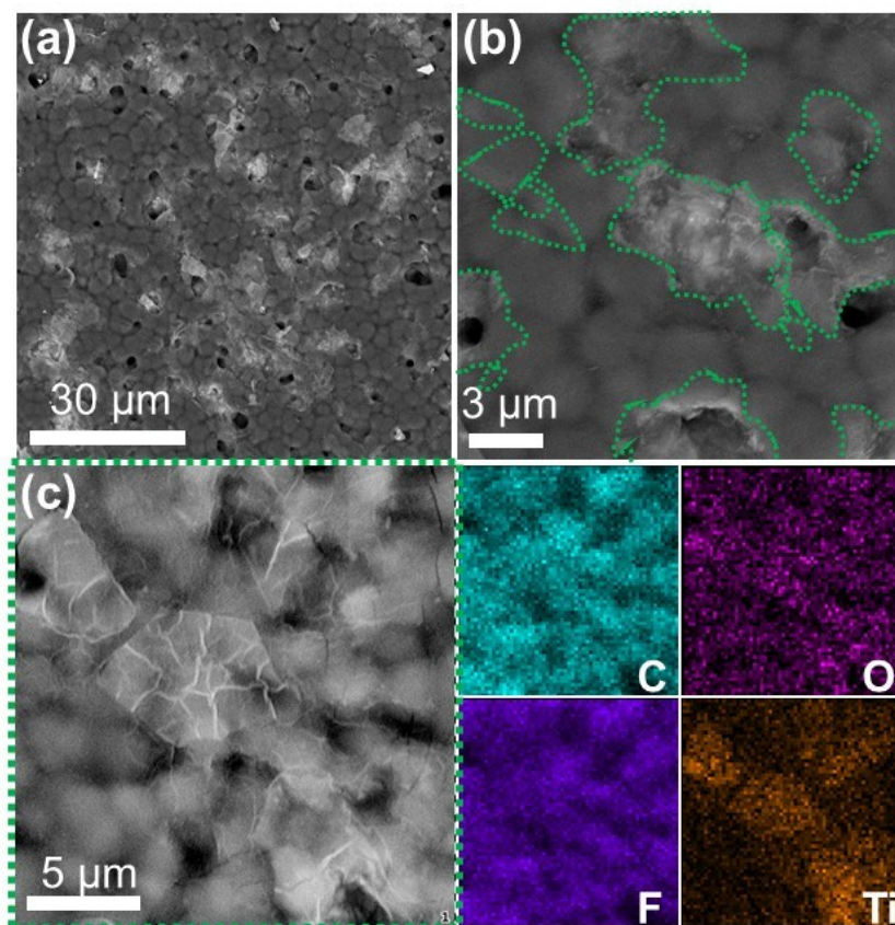
Fig. S1 Surface SEM images of MXene nanosheets on PVDF film with low (a) and (b) high magnification, where \text{Ti}_3\text{C}_2\text{T}_x nanosheets are marked with green dotted line. (c) The elements mapping images of carbon (C), fluorine (F), oxygen (O) and Titanium (Ti) in the area marked with green dotted line.
